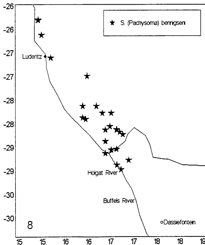
FIGS. 6-9. Distribution of Scarabaeus ( Pachysoma ) species in South Africa and Namibia. Questioned locality records or range extensions are shown by an open circle. (6) S. (P.) striatus ; (7) S. (P.) gariepinus ; (8) S. (P.) bennigseni ; (9) S. (P.) schinzi and S. (P.) valeflorae .
