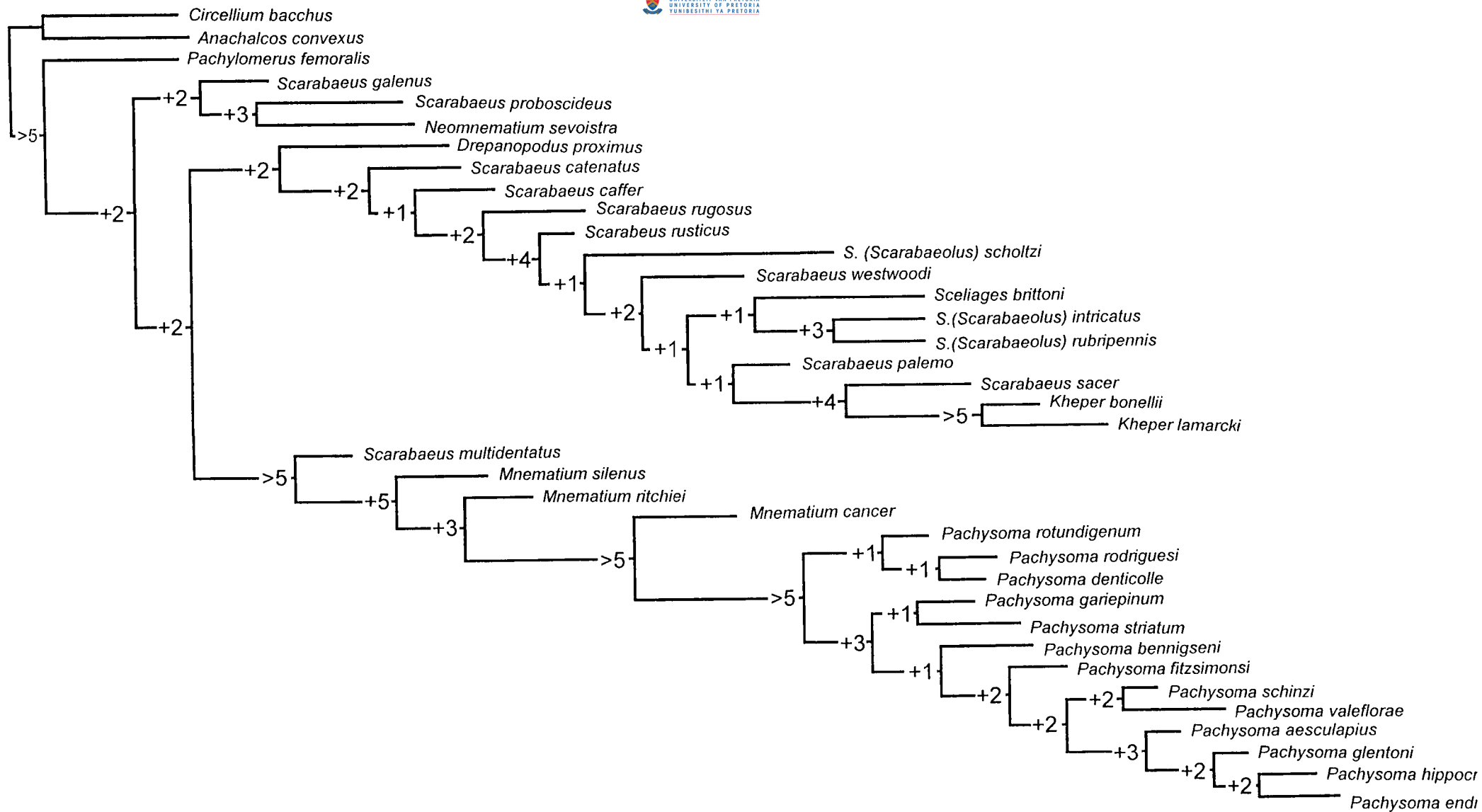
FIGURE 1. Cladogram depicting the relationship between the flightless Scarabaeini (i.e. Pachysoma , Neopachysoma , Mnematum and Neomnematum ) and representative taxa of the flying Scarabaeini genera (i.e. Scarabaeus , Kheper , Pachylomerus , Sceliages and Drepanopodus ) with Circellium and Anachalcos (tribe Canthonini) as outgroup taxa. The 823-step cladogram (C.I. = 0.52, R.I. = 0.85) was obtained after successive weighting of the 37 taxa and 64 characters. Decay Indices, i.e. the number of extra steps needed to collapse a node, are included at each node.
