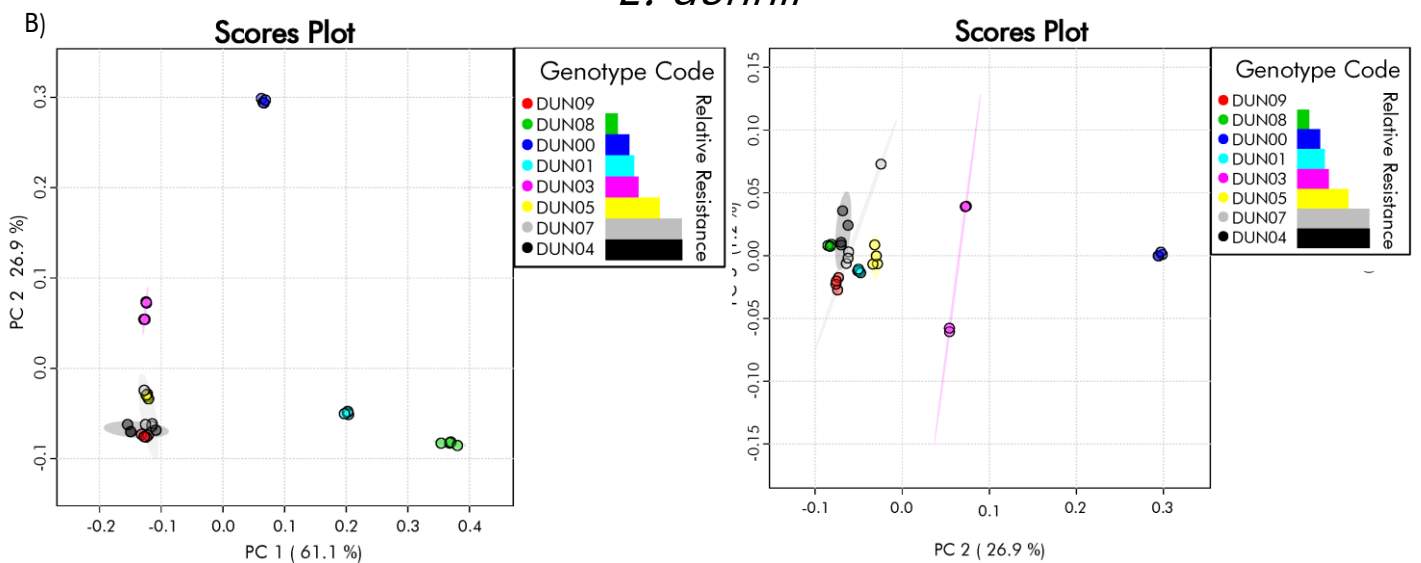
Figure 3: 2-Dimension principle component analysis of A) non-polar compounds found in E. grandis × urophylla leaves. B) non-polar compounds found in E. dunnii leaves. Horizontal bars indicate relative resistance of the clone to feeding by Gonipterus sp. n. 2 (relative to most susceptible tested genotype of its species (Dun09 and GU12))
