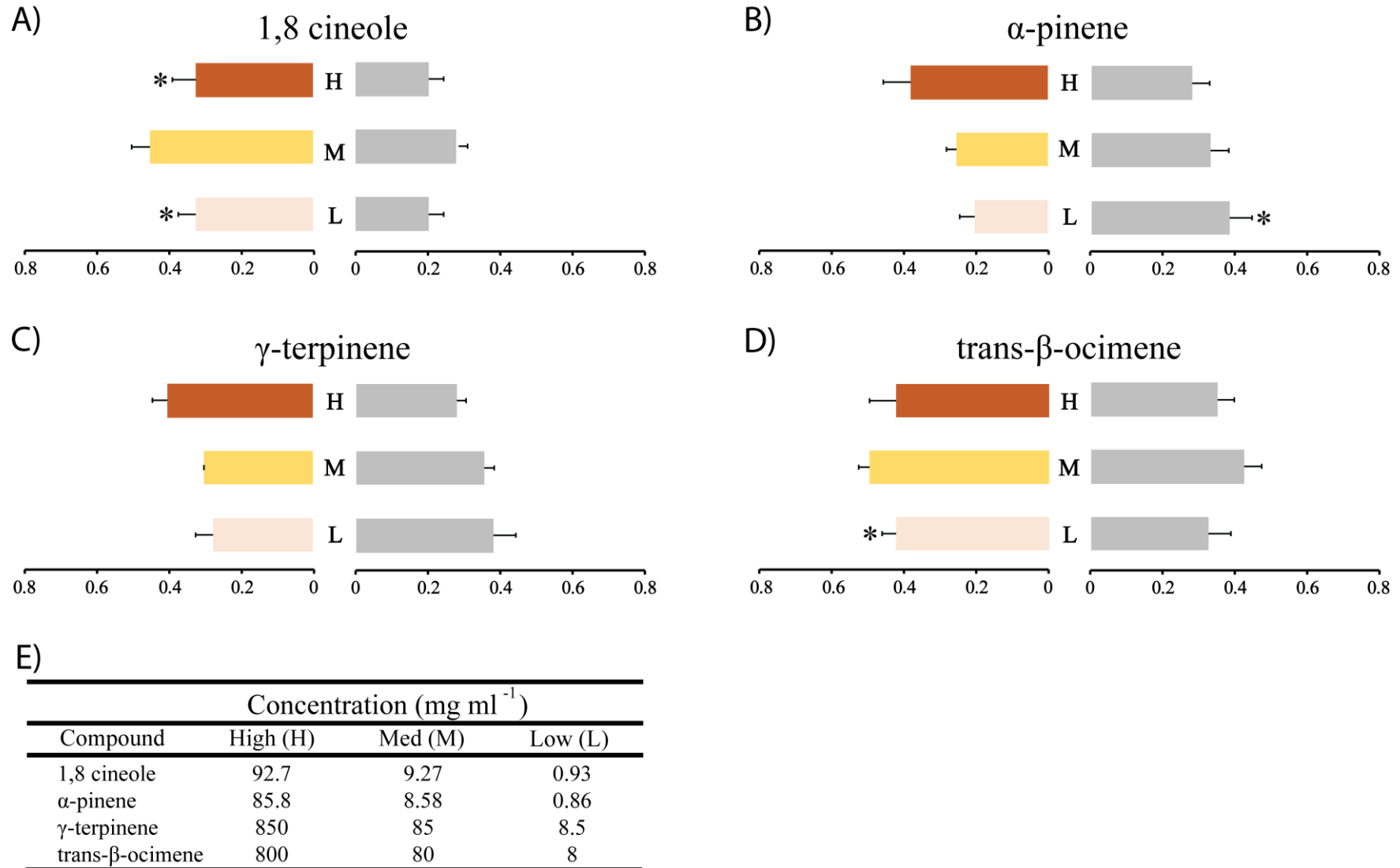
Figure 11: Weight of artificial diet consumed (g) comparing an unlaced artificial diet to an artificial diet laced with different concentrations of: A) 1,8 cineole B) α-pinene C) γ-terpinene D) trans-β-ocimene E) Concentrations of each compound used in the assays.
