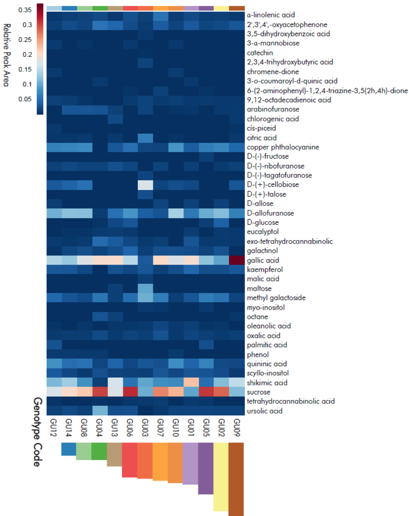
Figure 5: Heatmap of compounds with polar functional groups found in E. grandis x urophylla leaves. Vertical bars indicate relative resistance of the clone to feeding by Gonipterus sp. n. 2 (relative to most susceptible tested genotype (GU12)).
