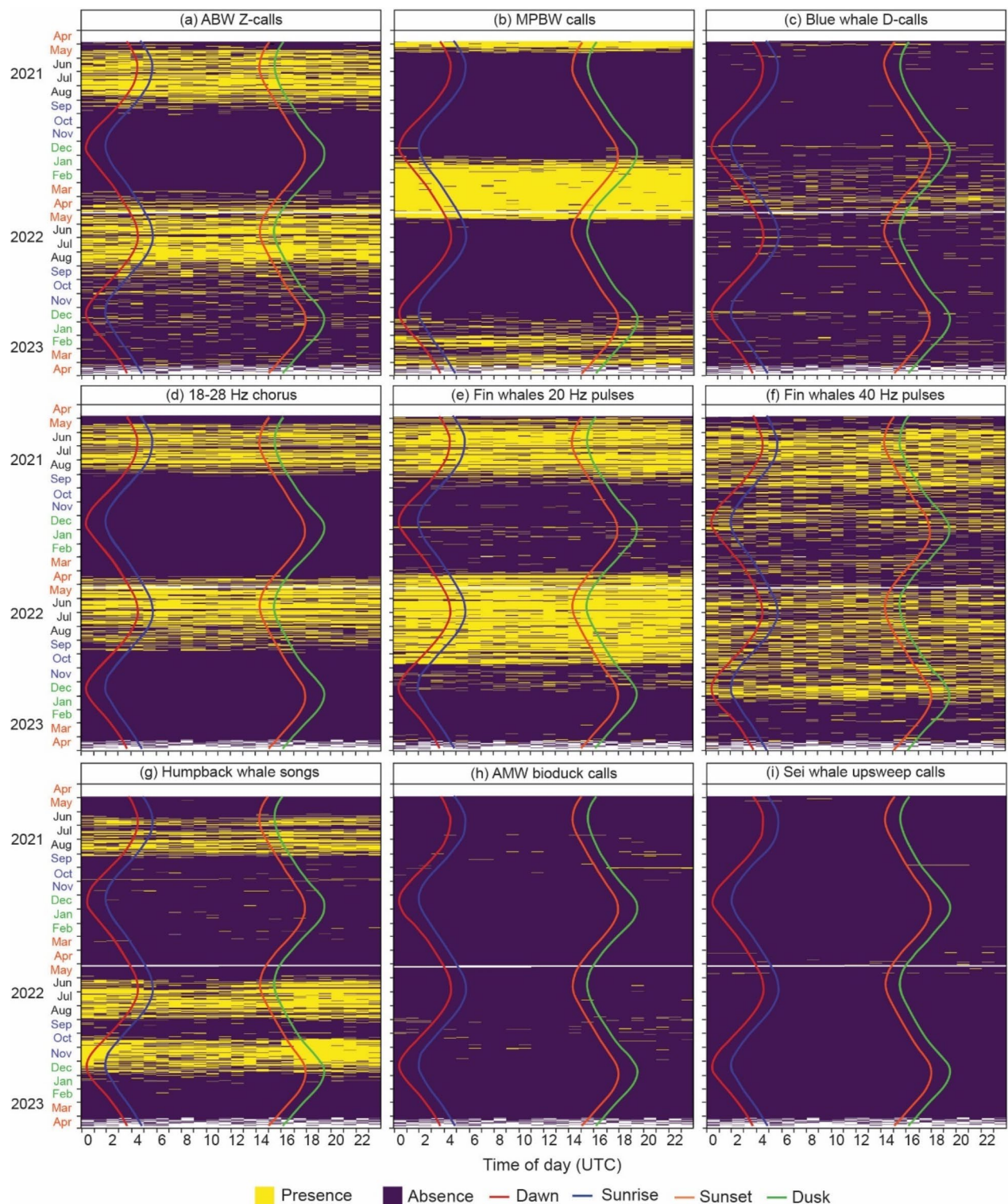
Fig. 4. Diel acoustic occurrence of different whale call types. Acoustic occurrence (i.e. absence/presence of calls) is defined in the key, and daylight regimes are indicated by vertical lines defined in the key. Month font colours represent seasons as defined above: green = summer, orange = autumn, black = winter, and purple = spring. White shading indicates periods without PAM effort, and the period of acoustic recorder malfunction in April 2023.
