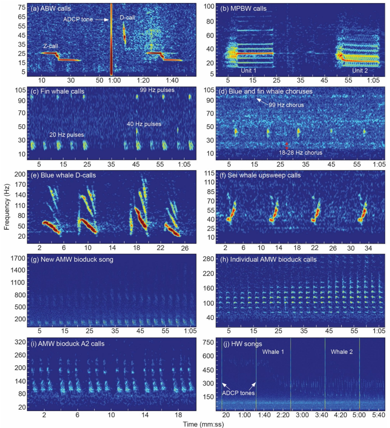
Fig. 2. Spectrograms showing (a) Antarctic blue whale (ABW) Z-calls, D-call, and ADCP tone; (b) Madagascan pygmy blue whale (MPBW) call units 1 and 2; (c) fin whale 20, 40, and 99 Hz pulses; (d) blue and fin whale 18–28 Hz chorus, 99 Hz chorus, and 40 Hz pulses; (e) blue whale D-calls with harmonics; (f) sei whale upsweep calls; (g) full frequency range including harmonics of Antarctic minke whale (AMW) bio-duck calls produced in song form; (h) zoom in below the 300 Hz range of (g) to show the spectral structure of the bio-duck call type described in this study; (i) AMW bio-duck A2 song; (j) humpback whale (HW) song from two whales singing simultaneously between regular ADCP tones. Note the different y-axes for each spectrogram. Parameters of each spectrogram (Hann window and 90% overlap were used to produce all spectrograms): (a) frame size = 1.75 s and discrete Fourier transform (DFT) size = 32,768 samples, (b) frame size = 1.24 s and DFT size = 16,384 samples, (c) frame size = 0.52 s and DFT size = 8,192 samples, (d) frame size = 0.93 s and DFT size = 16,384 samples, (e) frame size = 0.56 s and DFT size = 8,192 samples, (f) frame size = 0.60 s and DFT size = 8,192 samples, (g) frame size = 0.34 s and DFT size = 4,096 samples, (h) frame size = 0.70 s and DFT size = 8,192 samples, (i) frame size = 0.27 s and DFT size = 4,096 samples, and (j) frame size = 0.93 s and DFT size = 16,384 samples.
