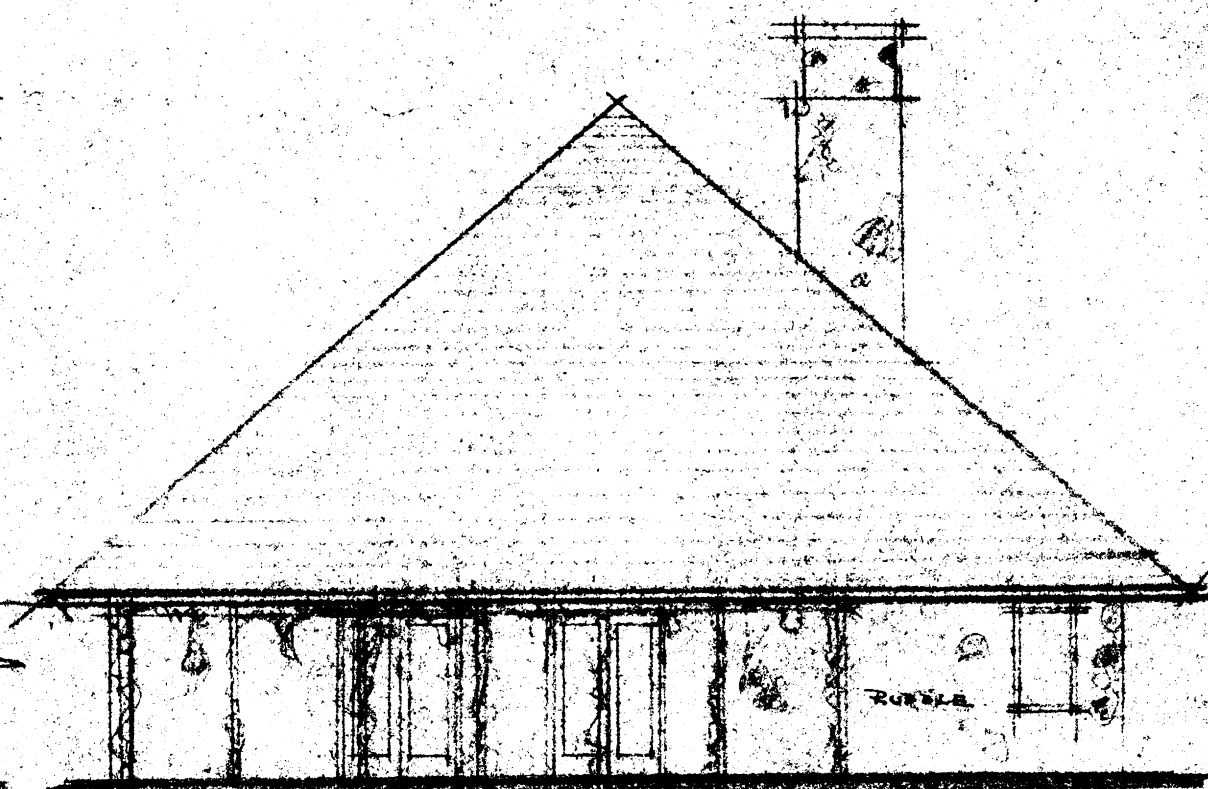
EAST ELEVATION
