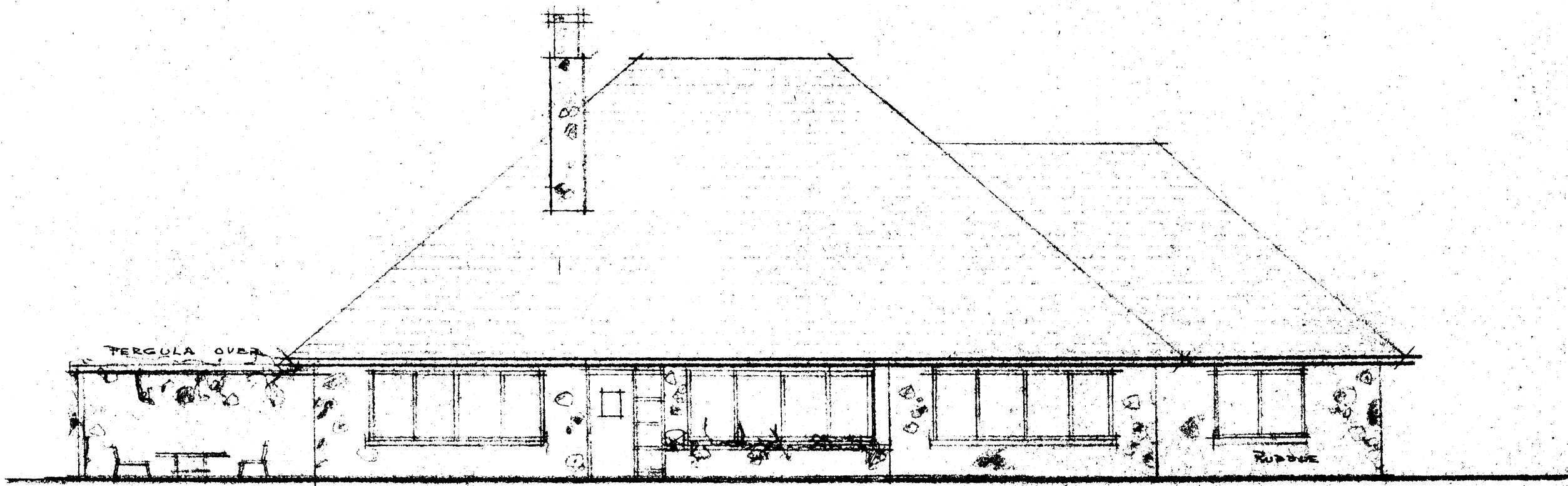
NORTH ELEVATION
