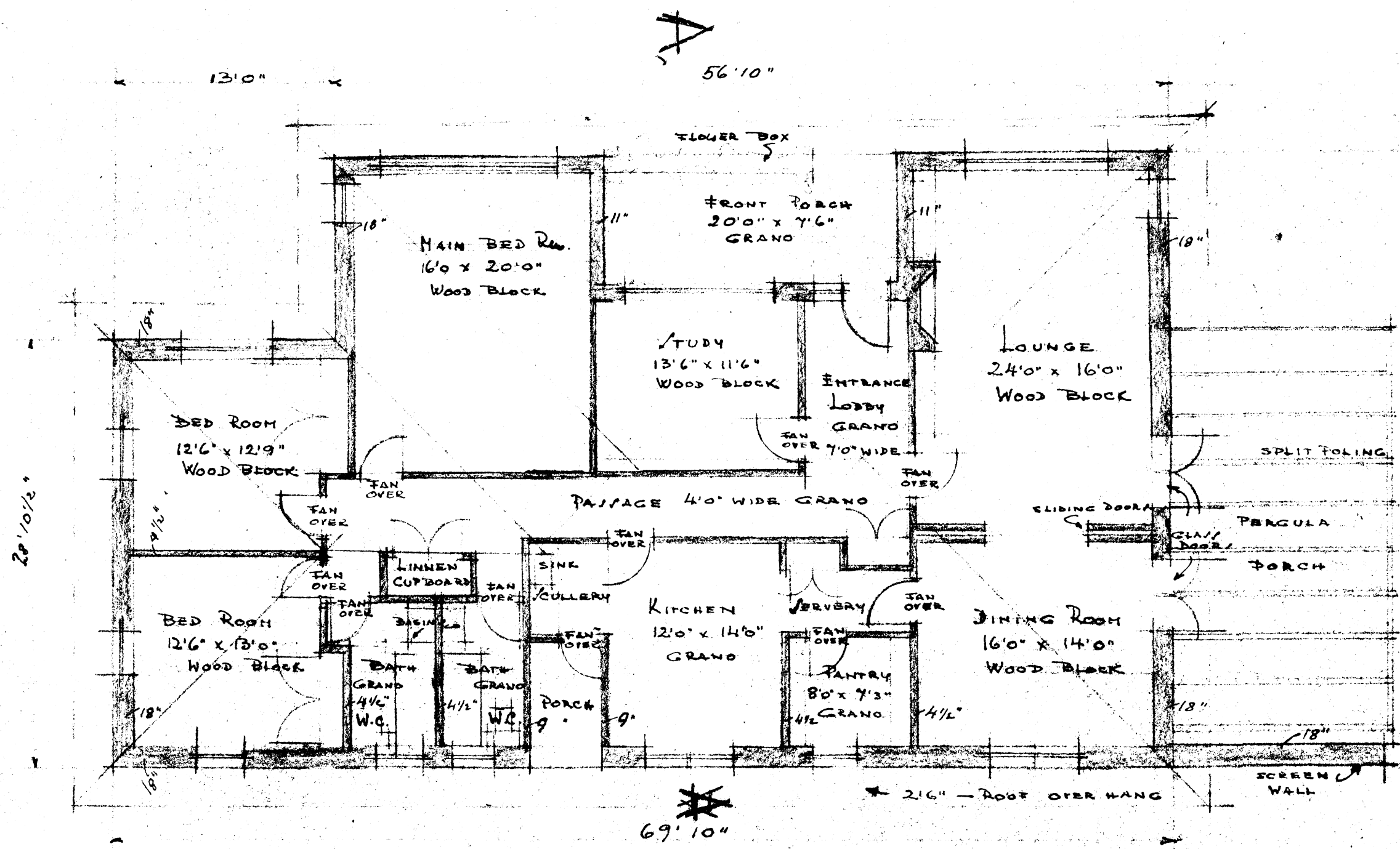
PLAN (SCALE 1 INCH = 8 FEET)
