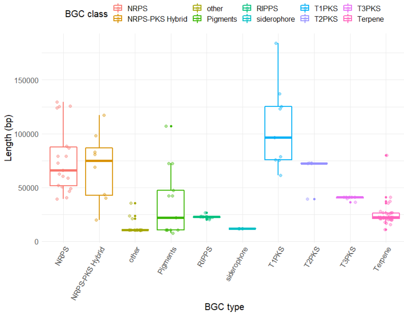
FIGURE S2 : Length (bp) of BGCs with a similarity score of 50% or greater to a known BGC in the MIBiG database (the same BGCs as in Fig. 3).
