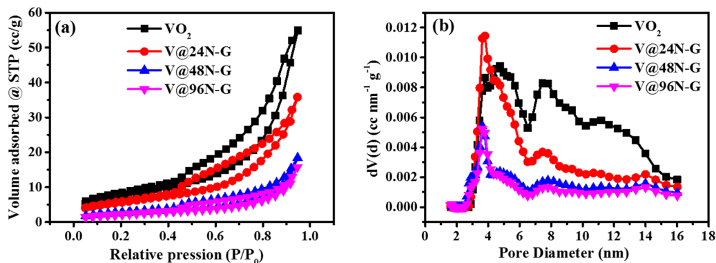
Fig. 2 (a) \text{N}_2 -adsorption/desorption isotherm curves and (b) PSD curves of \text{VO}_2 and V@XN-G nanocomposites.
