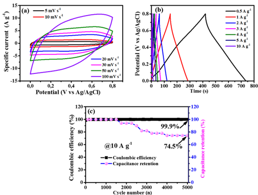
Fig. 7 (a) CV and (b) GCD profiles at different scan rates and specific currents, and (c) cycling stability test of V@48N-G up to 5000 GCD cycles.
