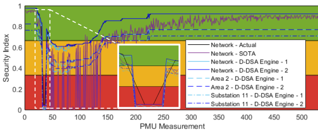
FIGURE 14. Security assessment index for TL1111L transmission line outage under Actual, SOTA, D-DSA Engine - 1 (Network, Area 2 and Substation 11) and D-DSA Engine - 2 (Network, Area 2 and Substation 11) approaches.
