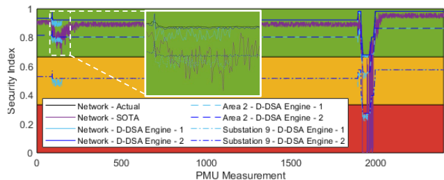
FIGURE 17. Security assessment index for extreme conditions simulated by considering both Substation 8 outage and TL1111L outage in sequence Actual, SOTA, D-DSA Engine - 1 (Network, Area 2 and Substation 9) and D-DSA Engine - 2 (Network, Area 2 and Substation 9) approaches.
