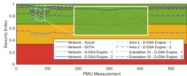
FIGURE 18. Security assessment index for TL54-53 transmission line outage under Actual, SOTA, D-DSA Engine - 1 (Network, Area 2 and Substation 53) and D-DSA Engine - 2 (Network, Area 2 and Substation 53) approaches.
