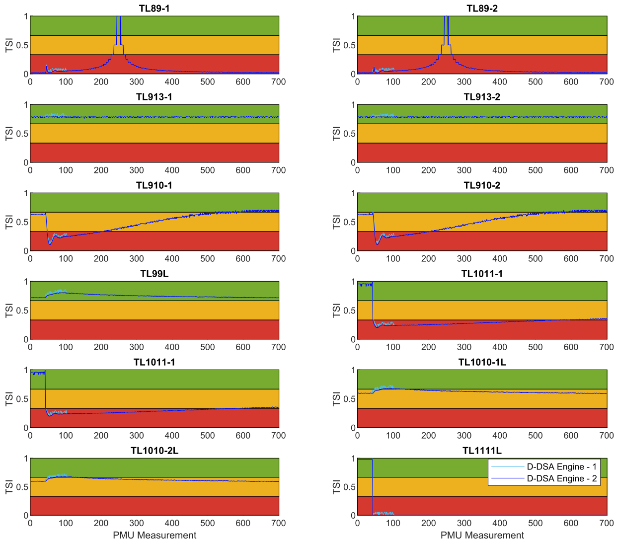
FIGURE 12. Transmission line security assessment index for TL1111L transmission line outage under D-DSA with D-LSE only and D-DSA with D-LSE and H-TNTP-PMU approaches. Area 2 Transmission Lines are presented.
