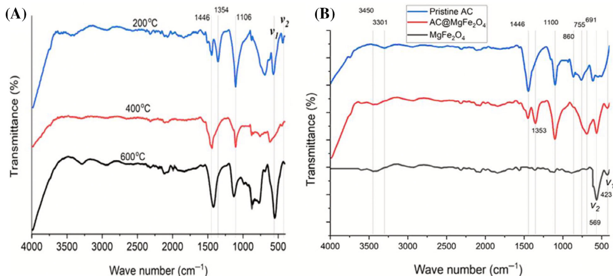
FIGURE 2 (A) Fourier transform infrared (FTIR) spectra of activated carbon-supported \text{MgFe}_2\text{O}_4 -layered double hydroxide ( \text{AC}@ \text{MgFe}_2\text{O}_4 -LDH) and the activated carbon-supported Mg-Fe layered double oxide ( \text{AC}@ \text{MgFe}_2\text{O}_4 LDO) calcined at different temperatures. (B) FTIR spectra of the pristine AC, \text{MgFe}_2\text{O}_4 , and \text{AC}@ \text{MgFe}_2\text{O}_4 calcined at 400^\circ\text{C} .
