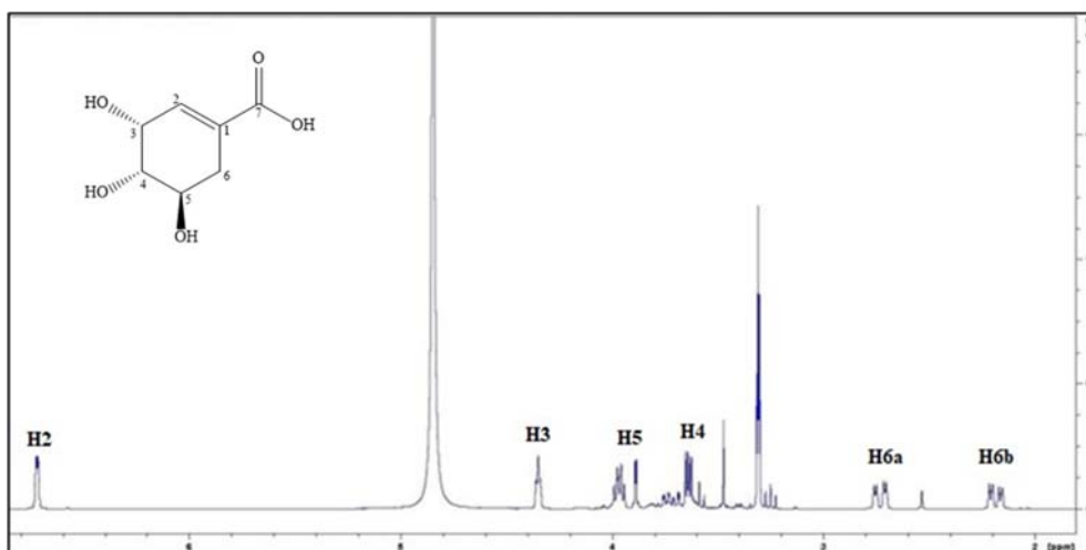
Figure S4. 1 H-NMR spectrum of compound 4 in CD 3 OD.
