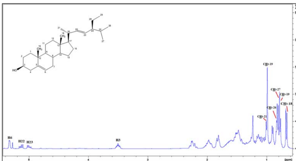
Figure S3. 1 H-NMR spectrum of compound 3 in CDCl 3 .
