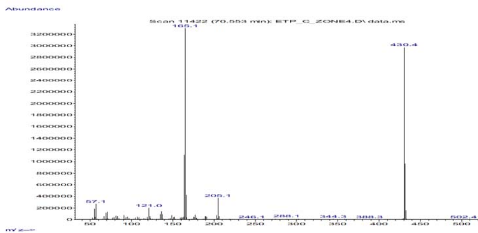
Figure S2. GC-MS of compound 2.
