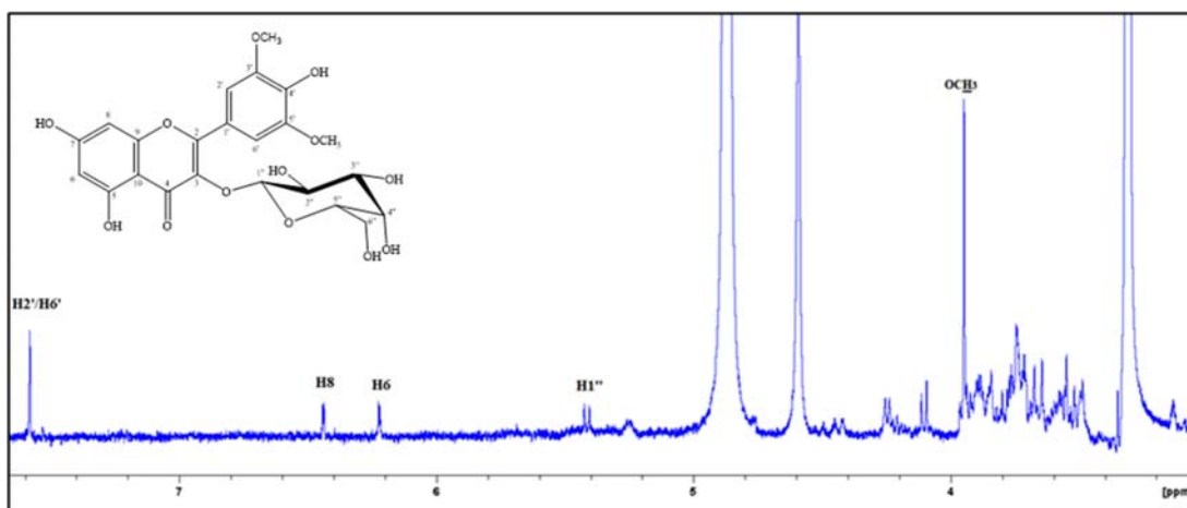
Figure S7. ^1\text{H-NMR} spectrum of compound 8 in \text{CD}_3\text{OD} .
