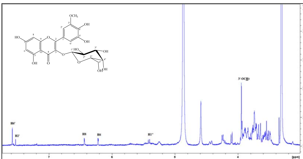
Figure S8. ^1\text{H-NMR} spectrum of compound 9 in \text{CD}_3\text{OD} .
