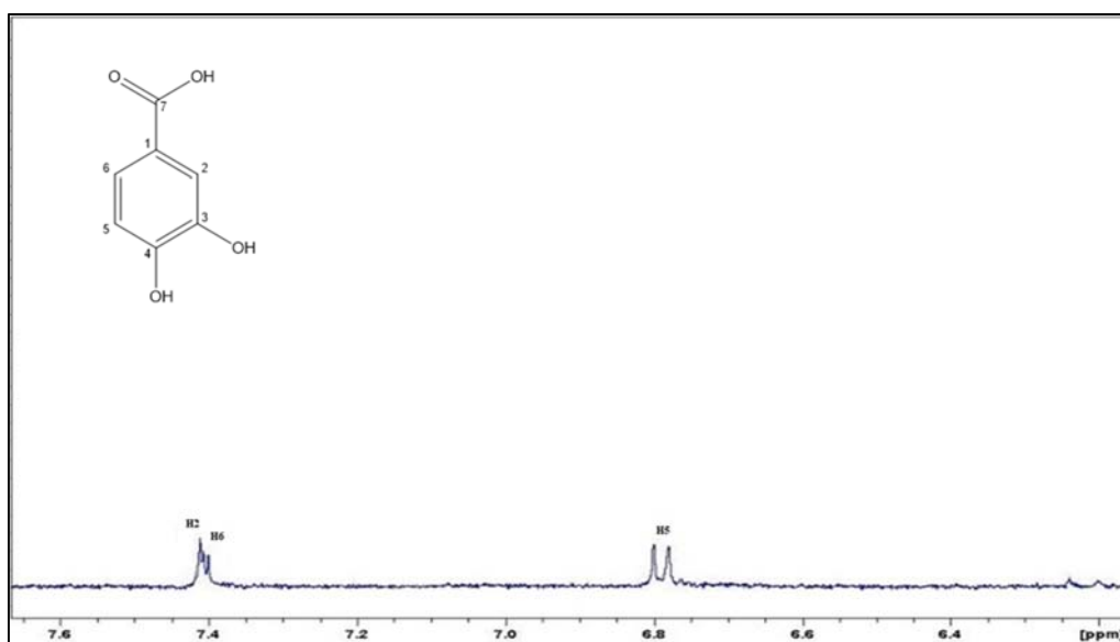
Figure S6. ^1\text{H} -NMR spectrum of compound 6 in \text{CD}_3\text{OD} .
