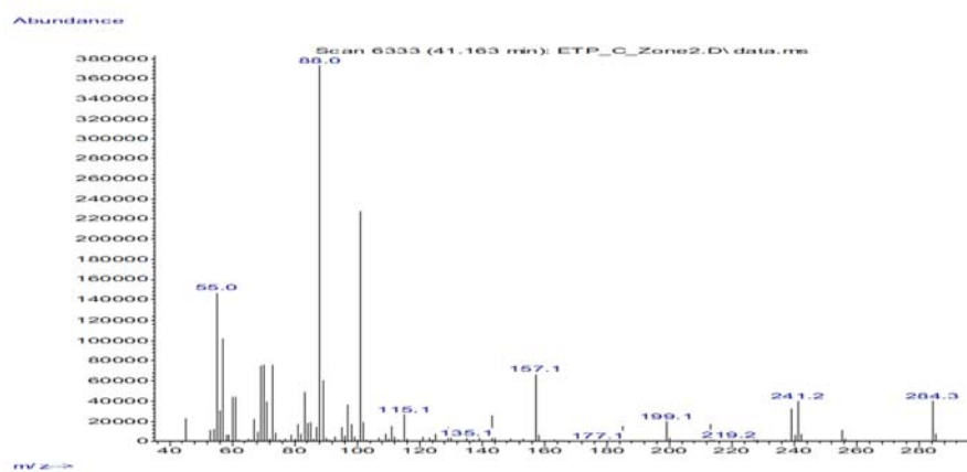
Figure S1. GC-MS of compound 1.
