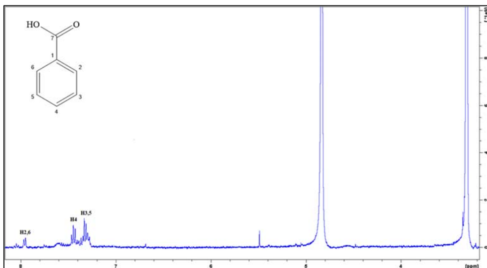
Figure S5. ^1\text{H} -NMR spectrum of compound 5 in \text{CD}_3\text{OD} .
