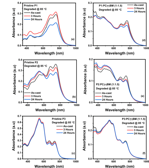
Fig. 1 Room-temperature absorption spectra of pristine terpolymers (a–c) and P1 – P3 :PC 71 BM thin films (d–f) degraded at 85 °C for 3 and 24 h.
