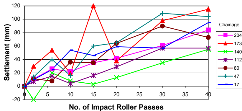
Figure 8. All settlement data.
