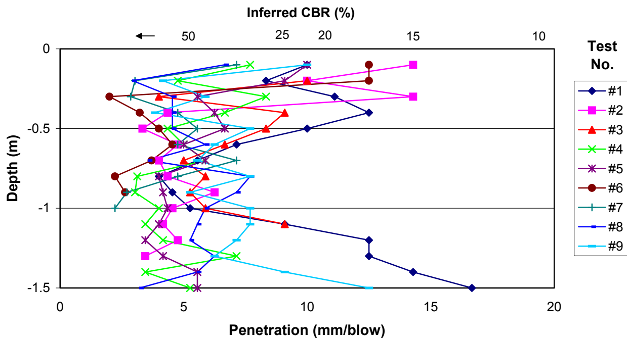
Figure 4. DCP Test Results.
