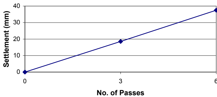
Figure 5. Average settlement on impact rolled platform.
