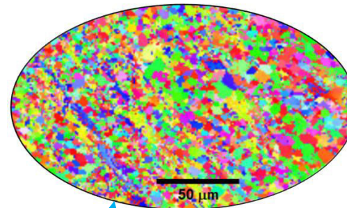
IPF at the optimum window
