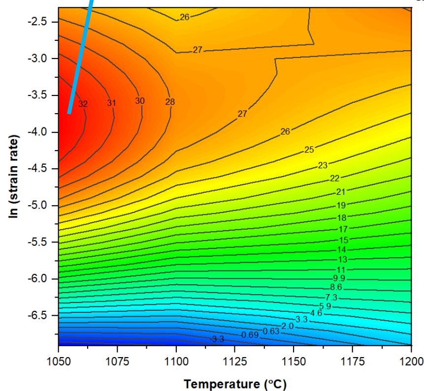
Power dissipation map
