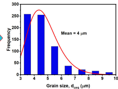
Grain size at the optimum window
