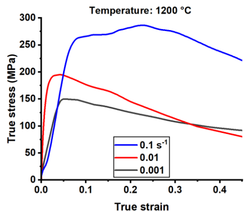
Hot compression flow curves
