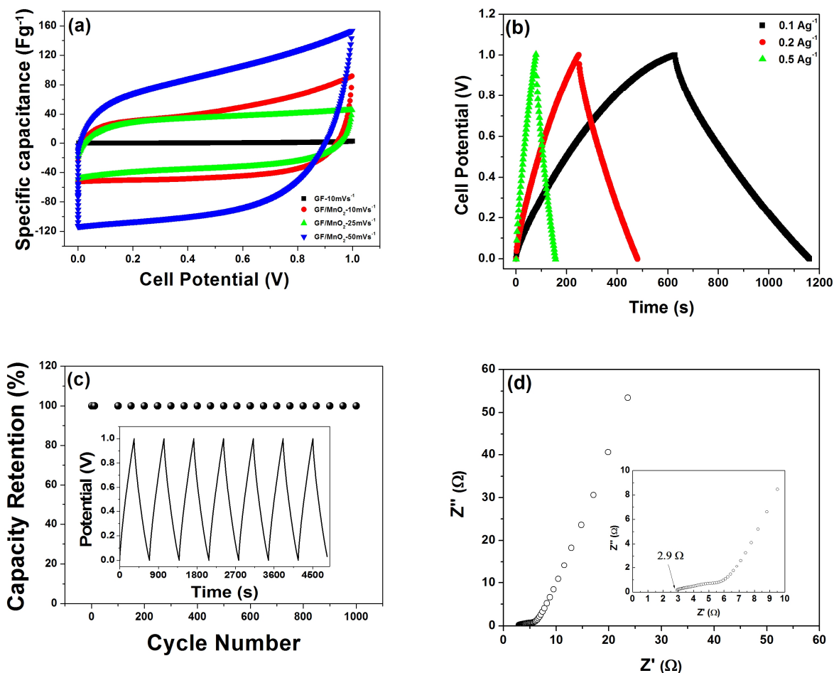
Figure 6 : Electrochemical characterizations of graphene foam/MnO 2 composites. (a) CVs of GF at scan rate of 10 mV/s and GF/MnO 2 composite at scan rates of 10, 25 and 50 mV/s. (b) the galvanostatic charge-discharge curves at three different current densities, (c) the capacity retention of the composite at a current density of 0.5 Ag -1 , inset shows the continuous charge-discharge curve, and (d) Nyquist plot for the GF/MnO 2 composite.
