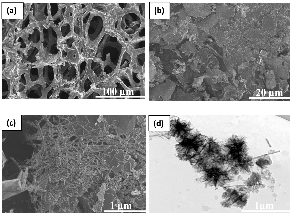
Figure 4 : SEM images of (a) graphene foam, (b, c) graphene foam/MnO 2 composite at different magnifications and (d) TEM image of the graphene foam/MnO 2 composite.
