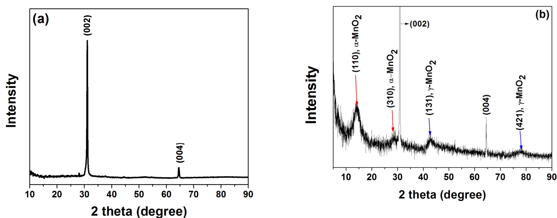
Figure 2 : XRD patterns of (a) graphene foam and (b) graphene foam/ \text{MnO}_2 composite.
