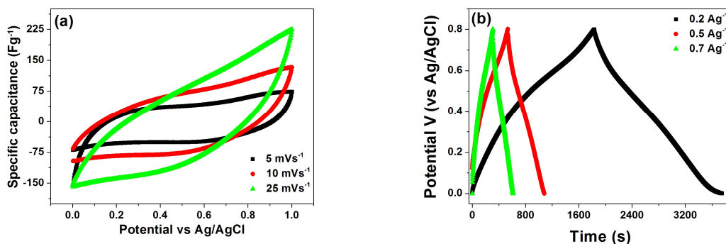
Figure 5 : Cyclic voltammetry curves of GF/MnO 2 measured at 5, 10 and 25 mVs -1 , (b) Galvanostatic charge-discharge profiles of GF/MnO 2 electrode at three different current densities in a three electrode configuration.
