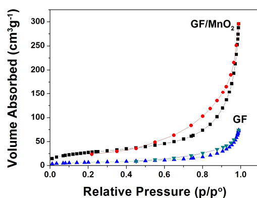
Figure 3 : Nitrogen adsorption and desorption isotherms for GF and GF/ \text{MnO}_2 composite.
