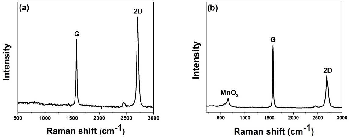
Figure 1 : Raman spectra of (a) graphene foam and (b) graphene foam/MnO 2 composite (GF/MnO 2 )
