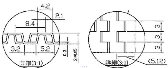
Figure 2 Geometrical configuration of the offset strip fins.
