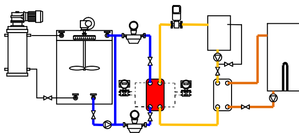
Figure 3 Schematic diagram of the experimental setup.
