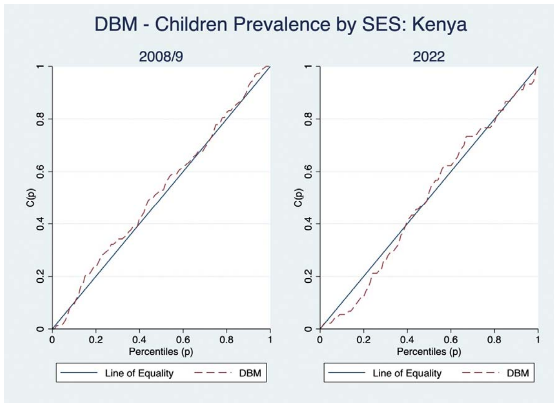
Supplementary: Figure 7; Lorenz Curves for DBM in under-fives for Kenya
