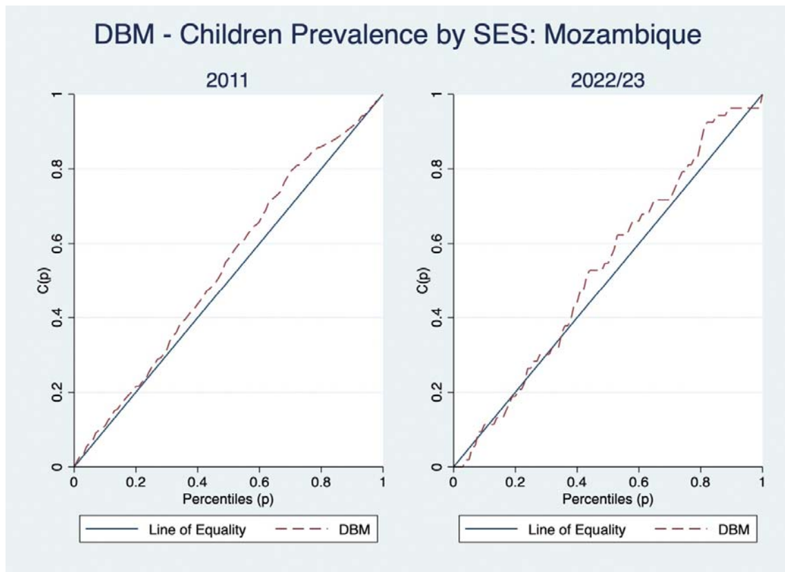
Supplementary: Figure 11; Lorenz Curves for DBM in under-fives for Mozambique
