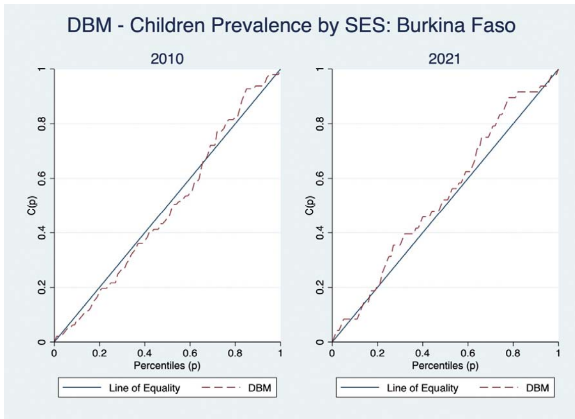
Supplementary: Figure 18; Lorenz Curves for DBM in under-fives for Burkina Faso
