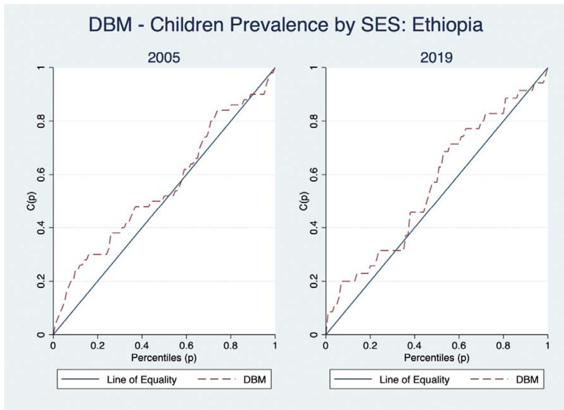
Supplementary: Figure 9; Lorenz Curves for DBM in under-fives for Ethiopia
