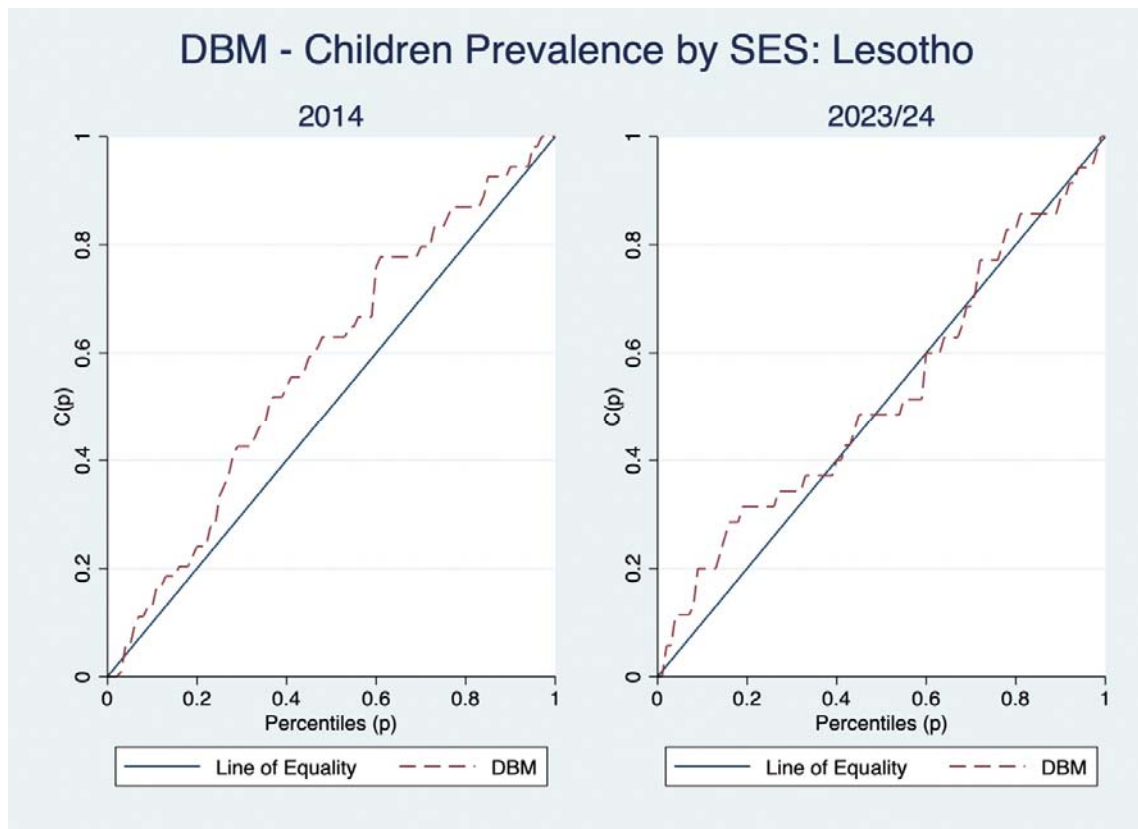
Supplementary: Figure 12; Lorenz Curves for DBM in under-fives for Lesotho
