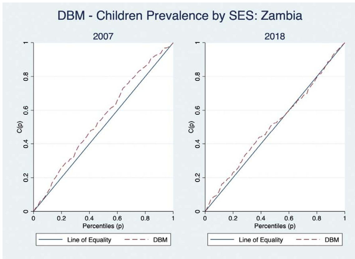
Supplementary: Figure 2; Lorenz Curves for DBM in under-fives for Zambia
