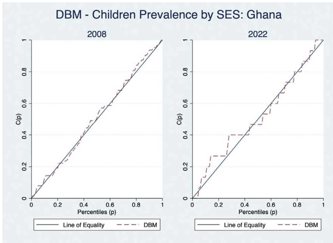
Supplementary: Figure 14; Lorenz Curves for DBM in under-fives for Ghana
