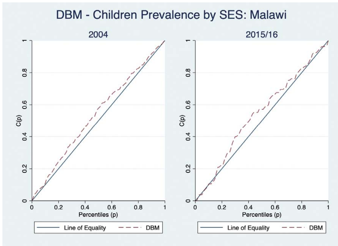
Supplementary: Figure 6; Lorenz Curves for DBM in under-fives for Malawi
