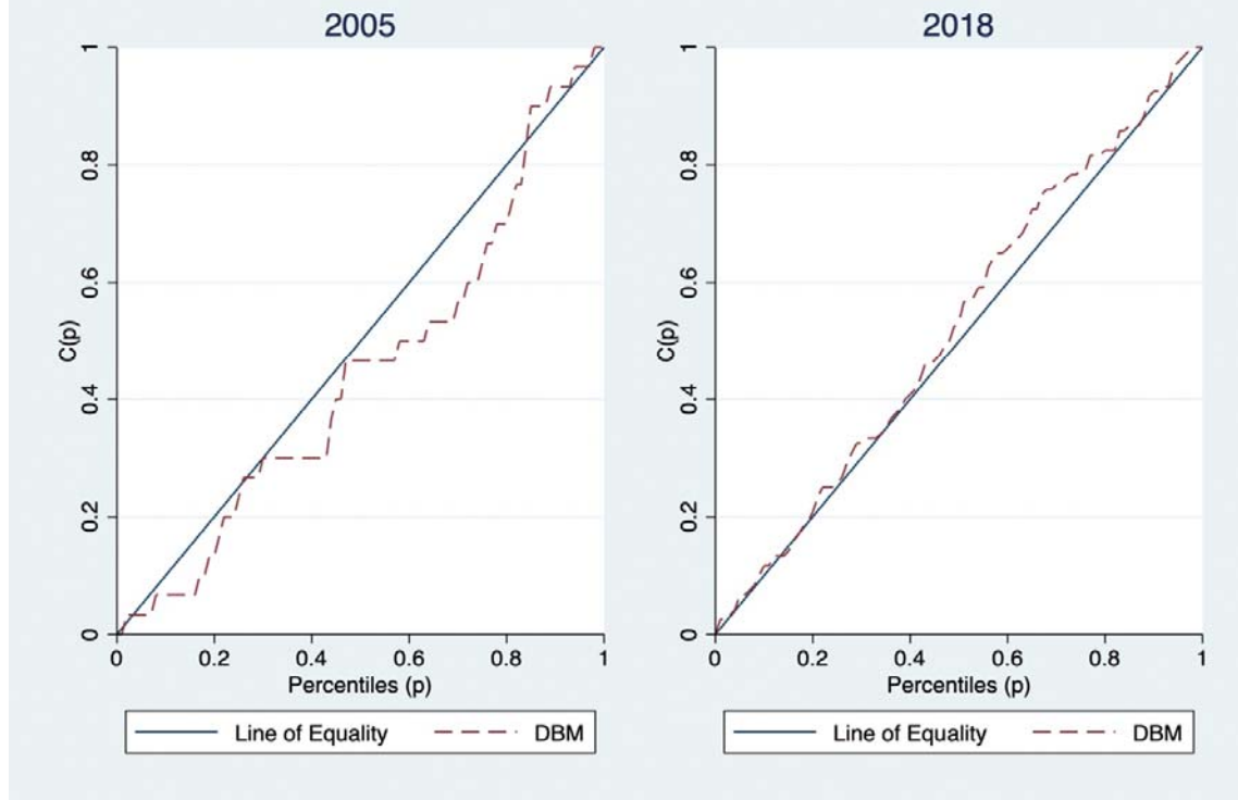
Supplementary: Figure 8; Lorenz Curves for DBM in under-fives for Guinea
