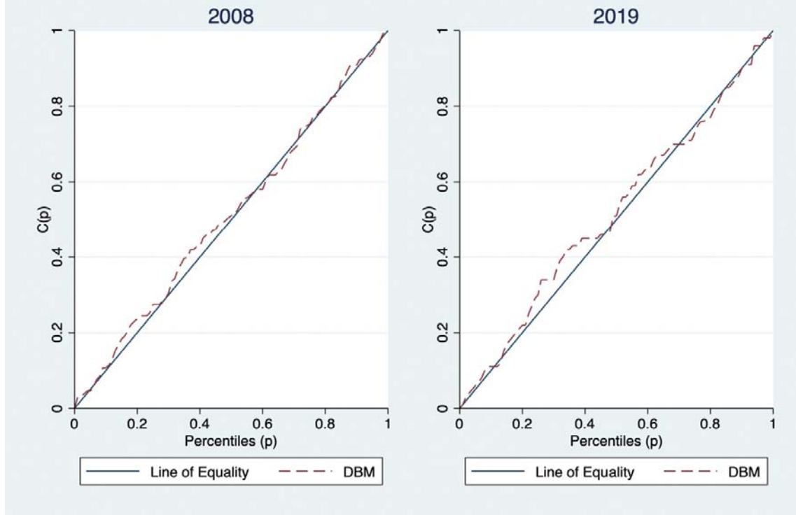
Supplementary: Figure 3; Lorenz Curves for DBM in under-fives for Siera Leone
