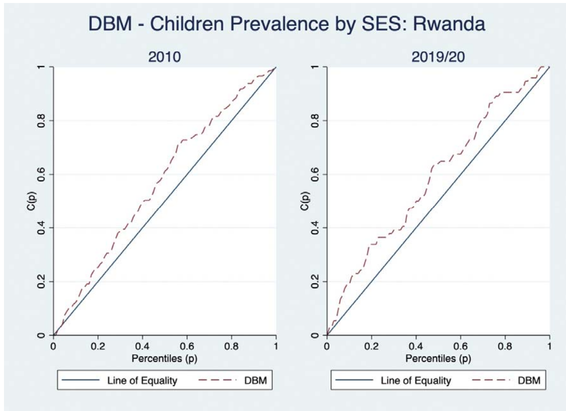
Supplementary: Figure 17; Lorenz Curves for DBM in under-fives for Rwanda
