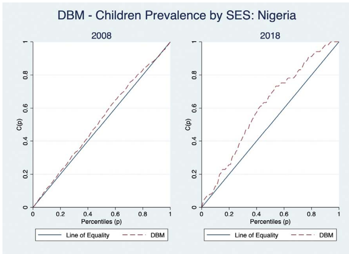
Supplementary: Figure 13; Lorenz Curves for DBM in under-fives for Nigeria
