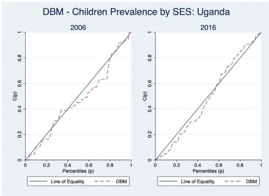
Supplementary: Figure 15; Lorenz Curves for DBM in under-fives for Uganda
