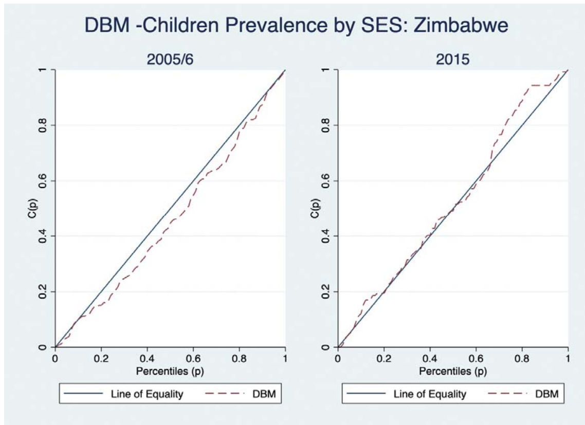
Supplementary: Figure 1; Lorenz Curves for DBM in under-fives for Zimbabwe
