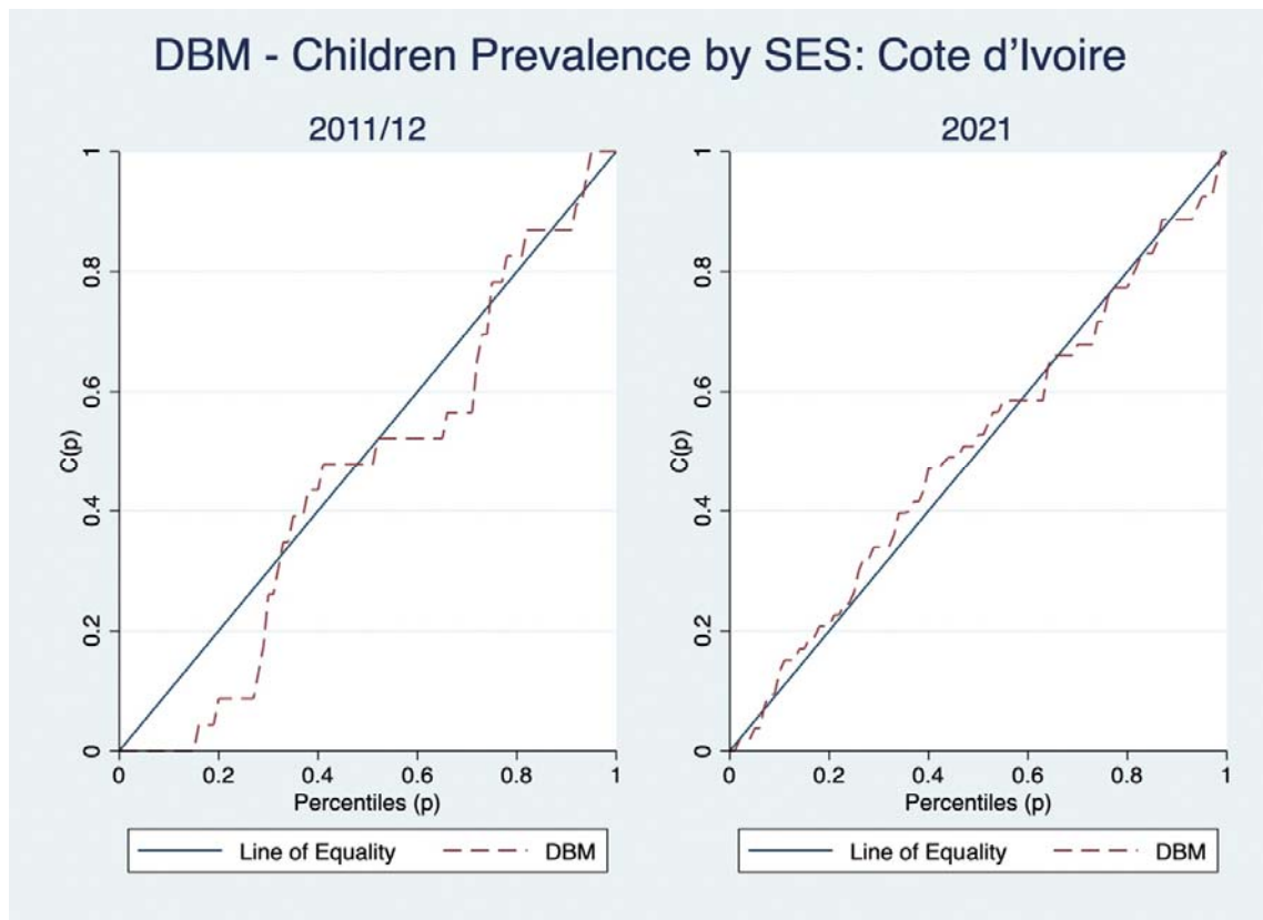
Supplementary: Figure 20; Lorenz Curves for DBM in under-fives for Cote d'Ivoire
