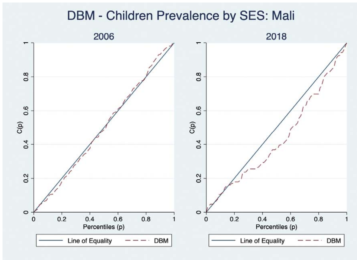
Supplementary: Figure 5; Lorenz Curves for DBM in under-fives for Mali
