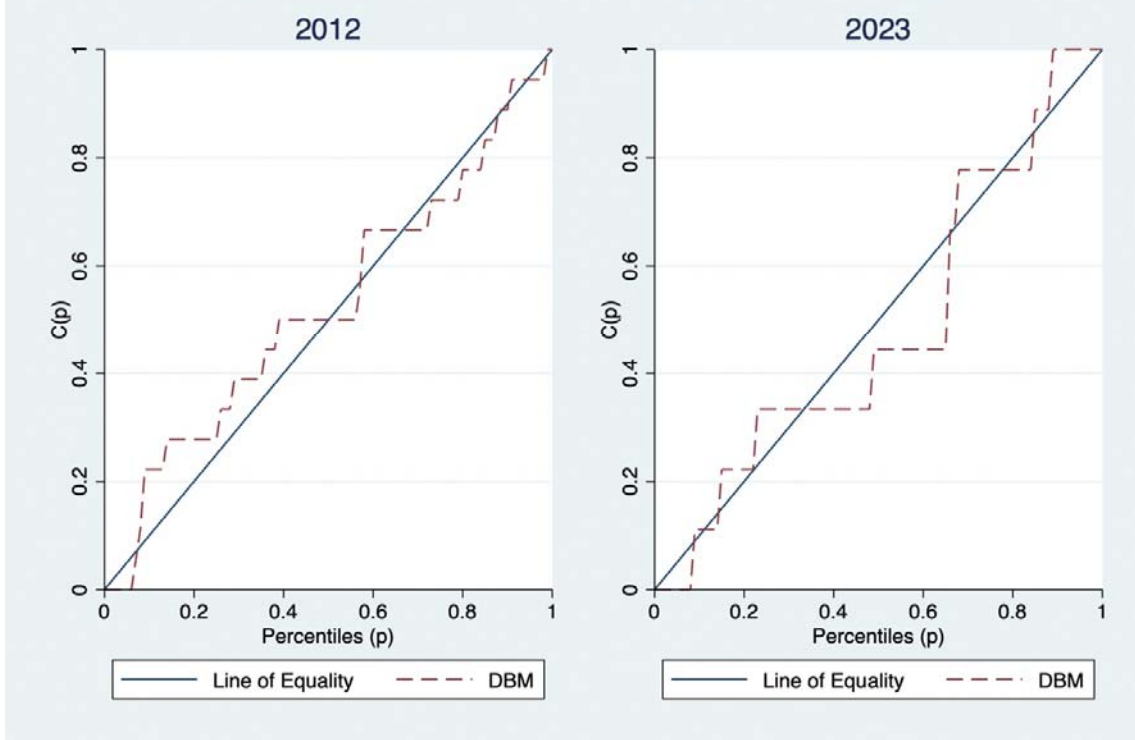
Supplementary: Figure 4; Lorenz Curves for DBM in under-fives for Senegal
