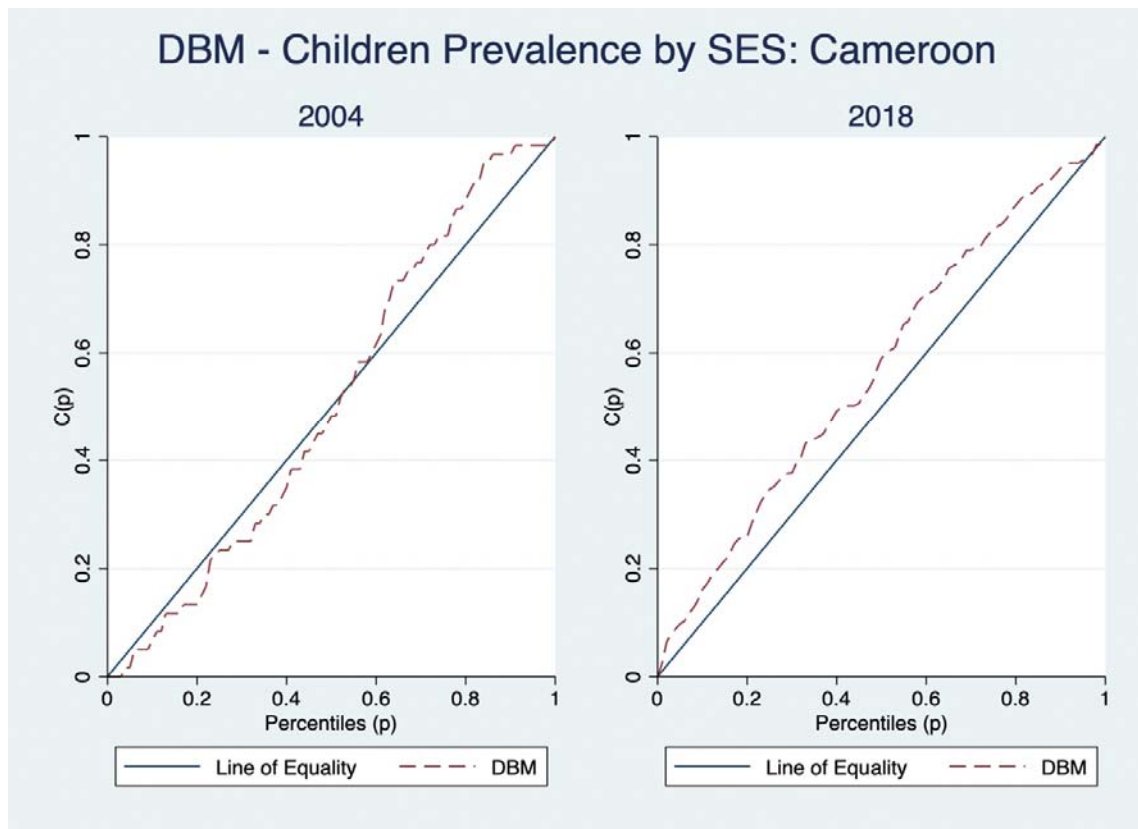
Supplementary: Figure 19; Lorenz Curves for DBM in under-fives for Cameroon
