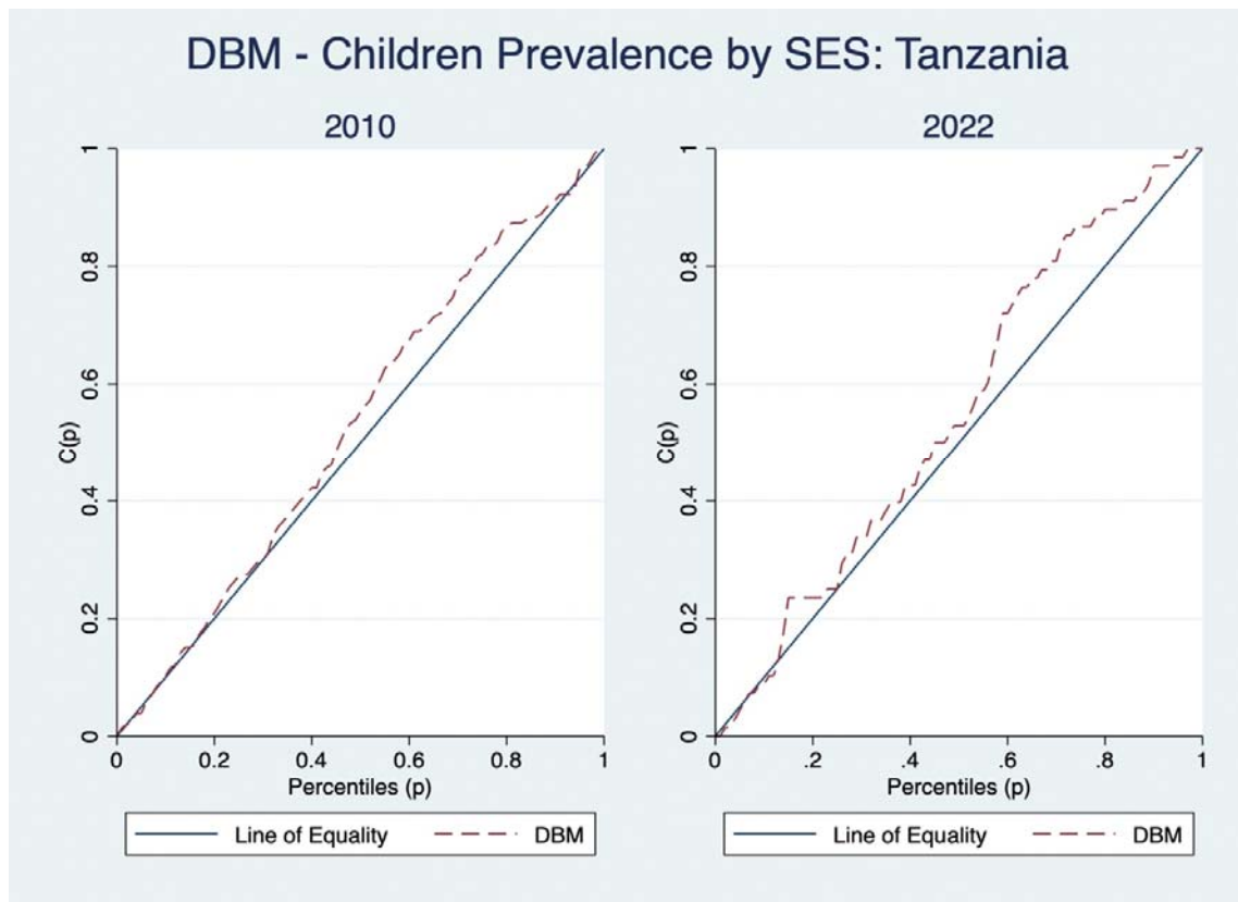
Supplementary: Figure 16; Lorenz Curves for DBM in under-fives for Tanzania
