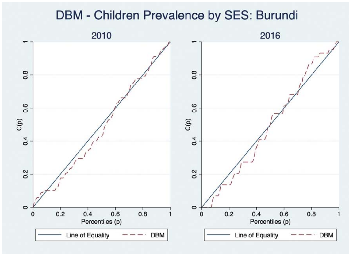
Supplementary: Figure 10; Lorenz Curves for DBM in under-fives for Burundi
