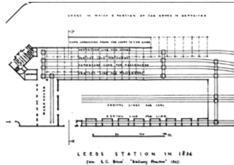
fig. 16_ Leeds station, 1834
