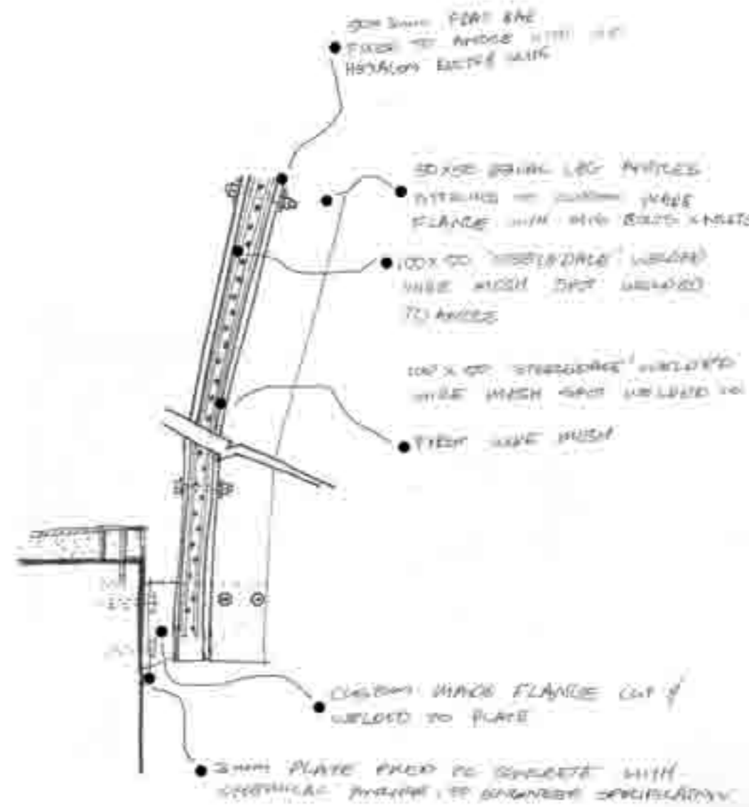
fig. 146_ Detail of platform enclosure, not to scale
