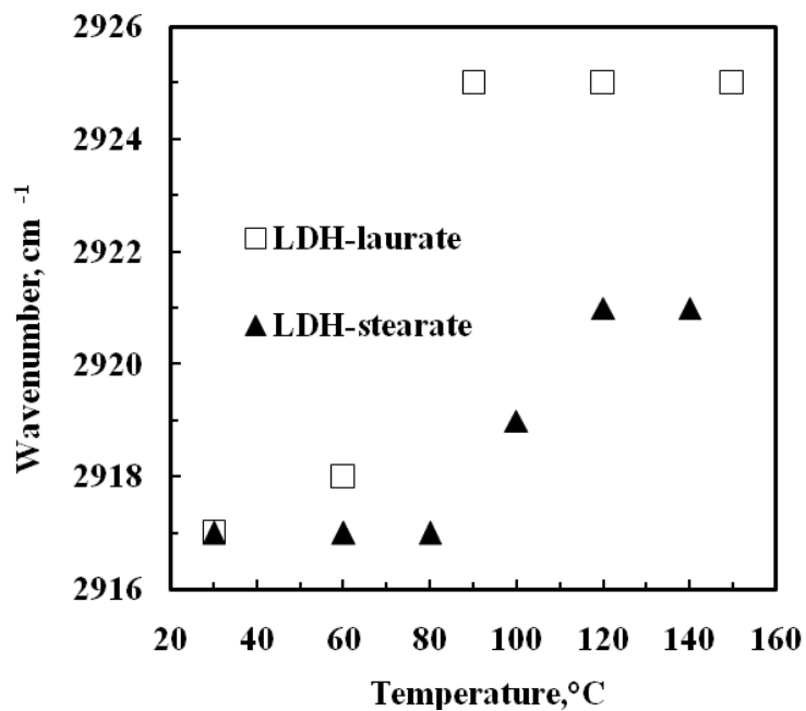
FIGURE 9 The effect of temperature on the peak position of the \nu_{as}(CH_2) band in the FT-IR spectra for LDH-laurate and LDH-stearate.
