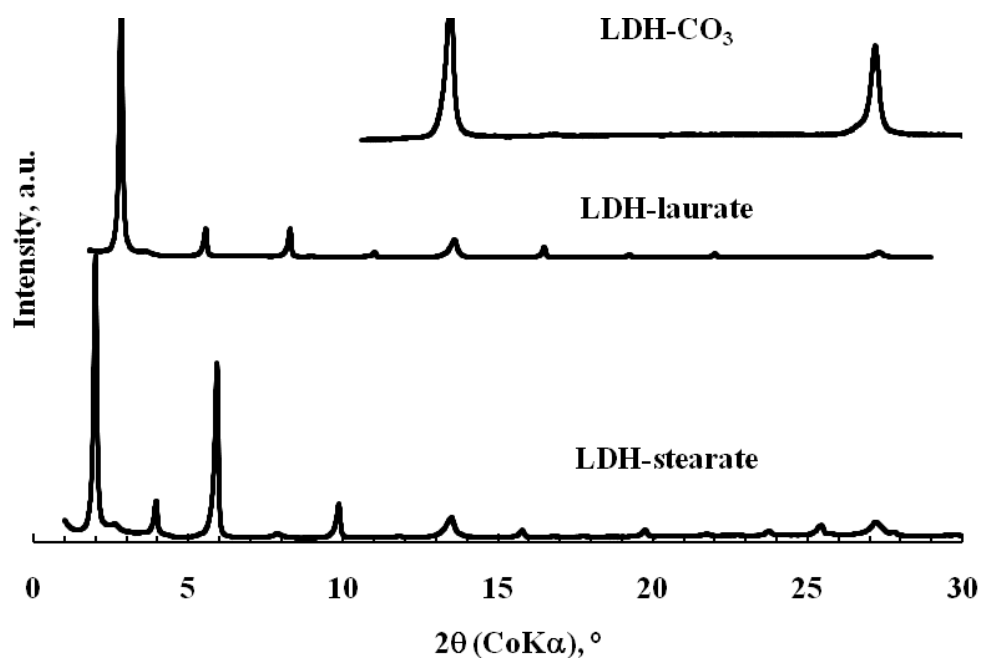
FIGURE 3 Powder XRD spectra for LDH-CO 3 , LDH-laurate and LDH-stearate.
