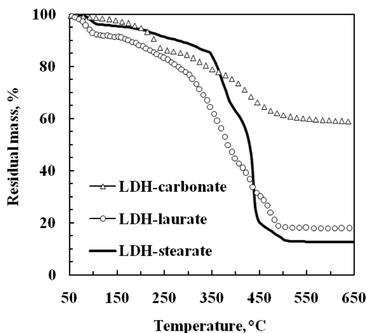
FIGURE 1 Thermogravimetric (TG) mass loss curves for LDH-CO 3 , LDH-laurate and LDH-stearate obtained at a scan rate of 10°C/min in an air atmosphere.
