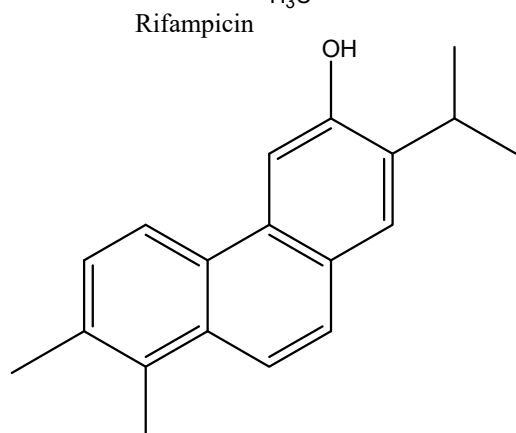
12-demethylmulticauline
