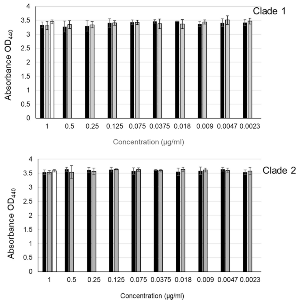
Fig. 3. Cytotoxicity studies in Vero cells validating both plants produced equine influenza clades 1 and 2. Results are shown for different concentrations of VLPs (black bars), and plant extract only (grey bars) compared to cells with WST-1 reagent (as control, white bar). The absorbance value is directly related to the amount of live, metabolically active cells present in each well.
