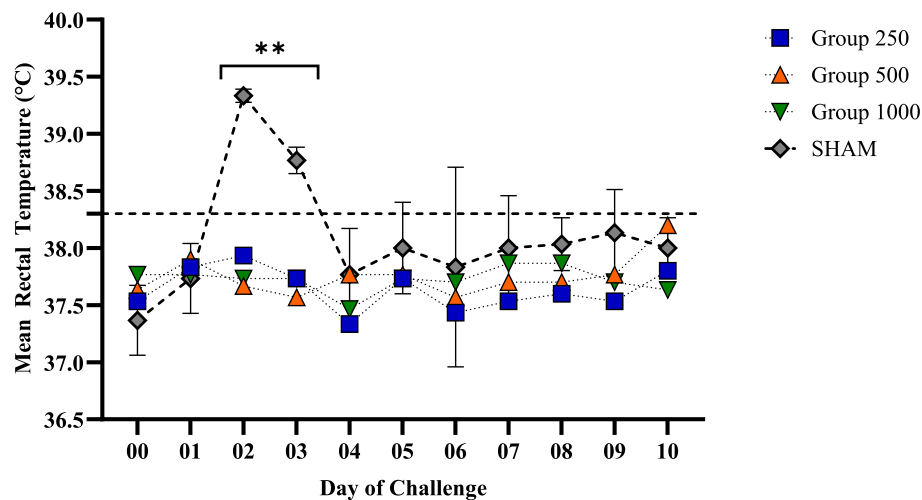
Fig. 4. Rectal temperatures of horses post-challenge. Days 0–10 correspond to D56–65 in text. Groups (250, 500, 1000, sham) correspond to the vaccine doses received. Shown are group means \pm SEM. Rectal temperatures >38.3^{\circ}\text{C} are considered pyrexia. Sham control group mean temperatures were significantly greater ( P < 0.01 ) than vaccine groups both Days 2 and 3, while rectal temperatures in all vaccinated horses remained within normal levels.
