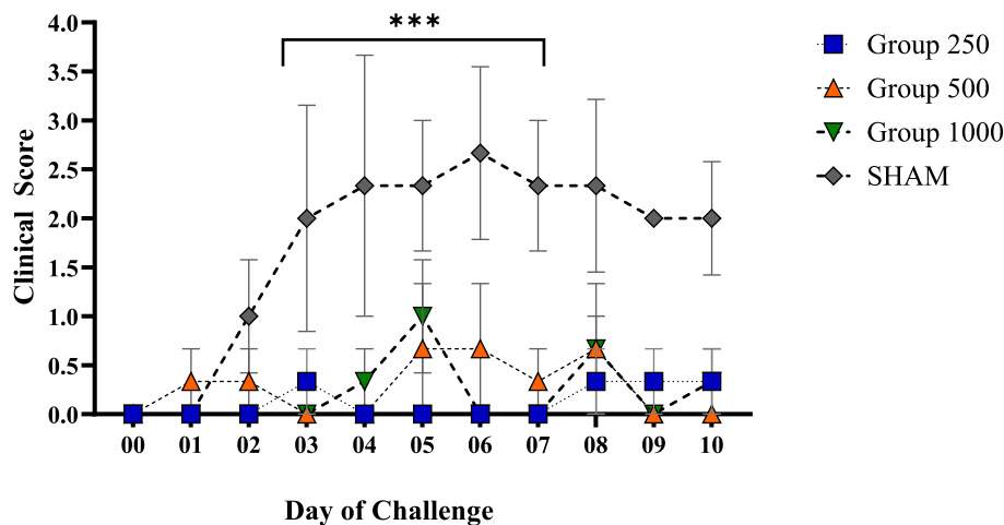
Fig. 5. Clinical scores of horses’ post-challenge. Days 0–10 correspond to D56–65 in text. Scores were calculated based on a Clinical Signs Scoring Index described previously (e.g. Blanco-Lobo et al., 2019). Groups (250, 500, 1000, sham) correspond to the vaccine doses received. Shown are group means \pm SEM. Scores for the sham group were significantly elevated over all vaccine groups on Days 3 through 7 ( p < 0.001 ). Clinical evaluations were done by an investigator blinded to the group assignments of the horses.
