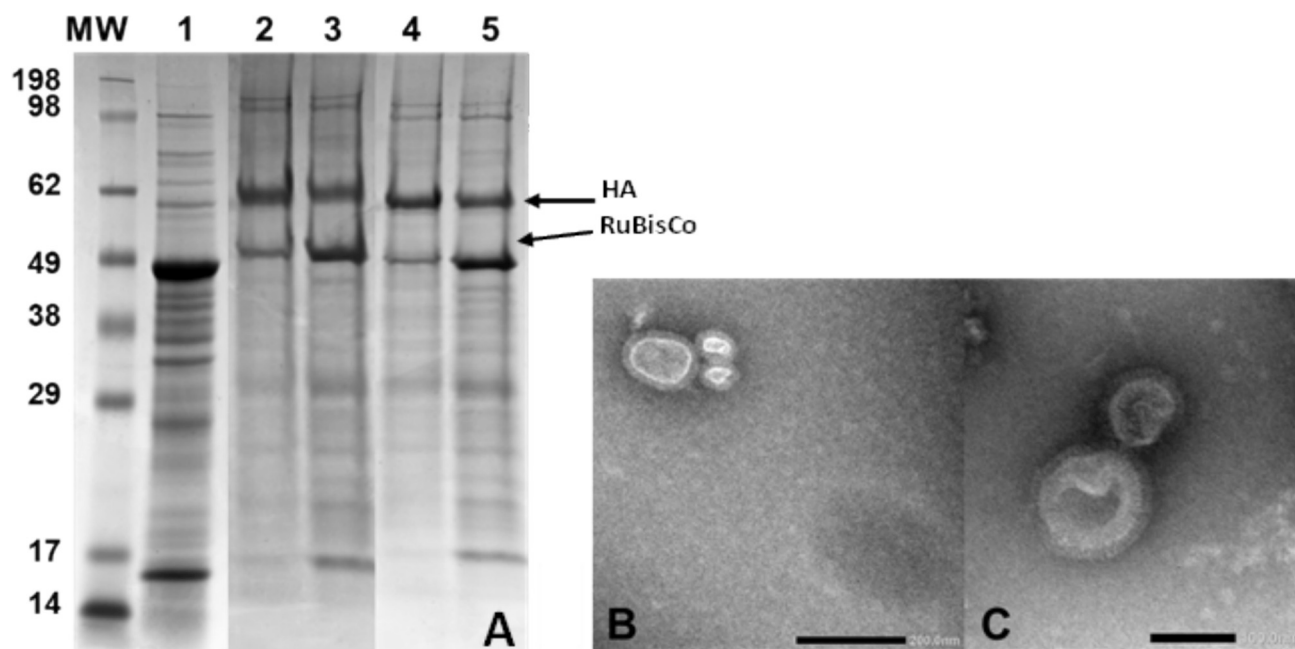
Fig. 2. A. SDS PAGE of plant-produced equine influenza clade 1 and 2 VLP proteins of 65 kDa in size (indicated by the arrow): See Blue® Plus2 pre-stained protein molecular weight marker (MW); lane 1, protein profile of plants agroinfiltrated with pEAQ-HT empty vector; protein profile of clade 1 (lanes 2–3) and clade 2 (lanes 4–5) purified from the TFF purified and filter sterilized sample using sucrose density gradient (70 % and 20 %) ultracentrifugation. B and C, negatively stained transmission electron microscopy (TEM) images of density gradient purified EIV FC1 and FC2 VLPs, respectively, measuring 80–120 nm diameter. B, 200 nm bar and C, 100 nm bar. (For interpretation of the references to colour in this figure legend, the reader is referred to the web version of this article.)
