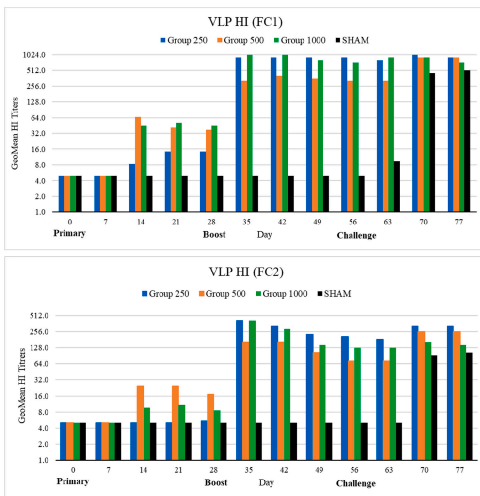
Fig. 1. Serology by HI testing of serum samples collected weekly (D0–77, with boost (second vaccine dose) on D28 and challenge on D56). Groups (250, 500, 1000, sham) correspond to the vaccine doses received. Shown are group mean HI titers; titers <10 (i.e. undetectable) are arbitrarily set to 5. Top panel, titers against Florida clade 1 (FC1) antigen (KY/14 virus strain). Bottom panel, titers against FC2 antigen (eq/Richmond/07 virus strain).
