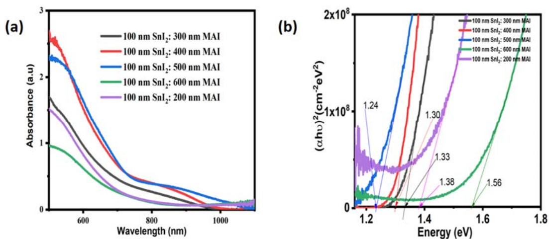
Figure S 1(a) U-V-vis absorption of MASnI 3 films with different thickness of MAI
