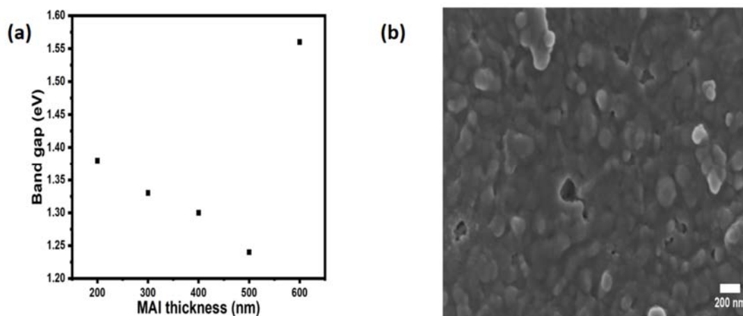
Figure S 2 (a) Plot of bandgap variation versus MAI thickness (b) SEM image of MASnI 3 film with 600nm MAI thickness
