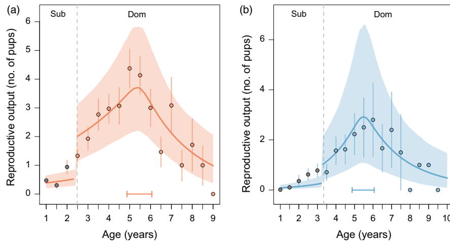
FIGURE 2 Age-related variation in reproductive output in female [red, (a)] and male [blue, (b)] meerkats. Solids lines display the predicted number of pups produced to emergence during each 6-month period for individuals who acquire dominance. The upper and lower limits of the coloured shaded areas show the 95% Bayesian credible intervals (BCI) estimates of the chronological age effect based upon fixed effects uncertainty. The 95% BCI of the threshold estimates are shown by the horizontal error bars. Predictions were made either side of the population mean age of dominance acquisition period (vertical striped line), with predictions representing subordinate reproductive output before this age and dominant reproductive output after. For predictions, rainfall and group size were set at the mean, longevity was set at 7 years, and season was set as 'second' (April–September). Points display the raw data with vertical error bars indicating \pm 1 SEM. Points are coloured to emphasize that, on average, most of the raw data prior to the vertical line come from individuals while they are subordinate (dark grey), whereas after this point, most data come from individuals that are dominant (red/blue)
