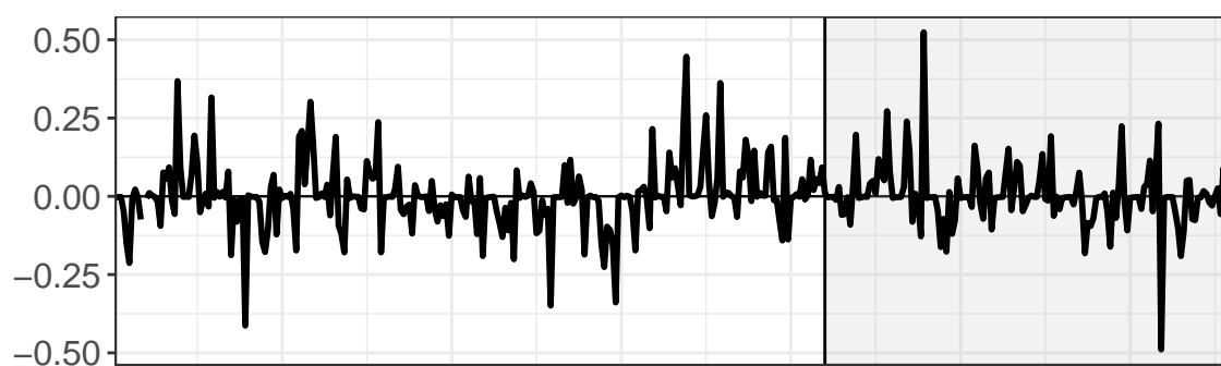
MIZ extent anomaly ( \text{km}^2 \times 10^6 )
