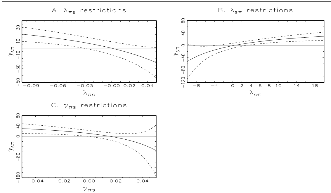
Figure 1: \gamma_{s\pi} estimates for different assumed \lambda_{\pi s} , \lambda_{s\pi} and \gamma_{\pi s} values
