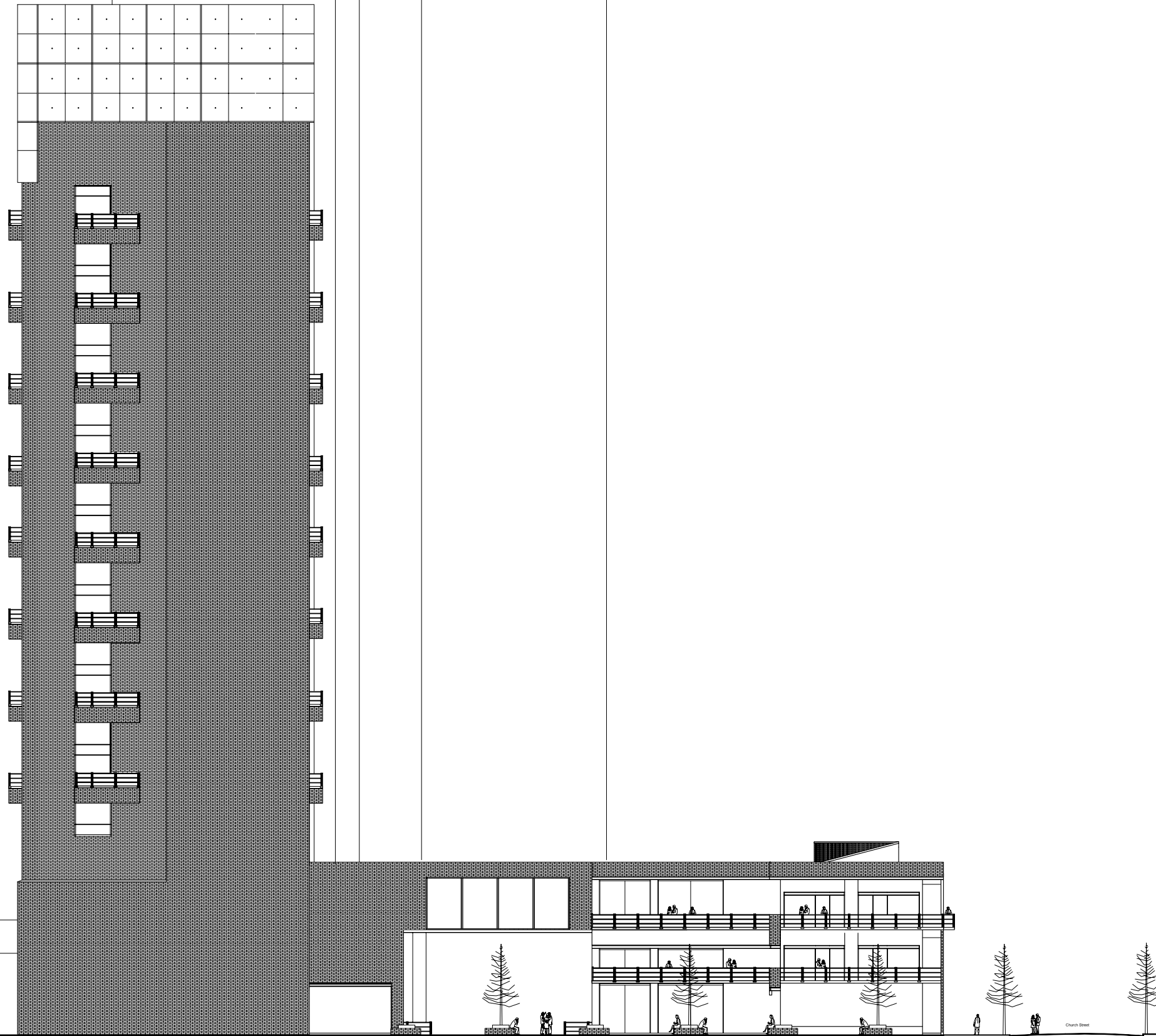
WEST - ELEVATION
