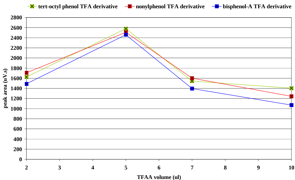
Figure 6.31 Optimum TFAA reagent volume, determined by placing 1 \mu\text{l} 42 ng/ \mu\text{l} TOP, 44 ng/ \mu\text{l} NP and 54 ng/ \mu\text{l} BPA in acetone on the PDMS trap; the corresponding reagent volumes are added after the solvent has evaporated. The trap is then sealed with glass caps for 10 minutes before thermal desorption and analysis. The optimum TFAA volume of 5 \mu\text{l} was visually determined from the x-y scatter plot as the point where maximum derivative peak area is observed.
