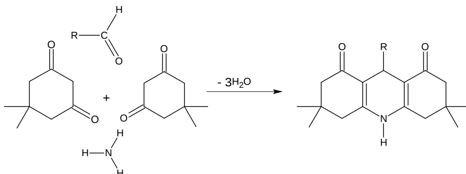
Figure 3.12 Hantzsch reaction scheme [156, 157].
