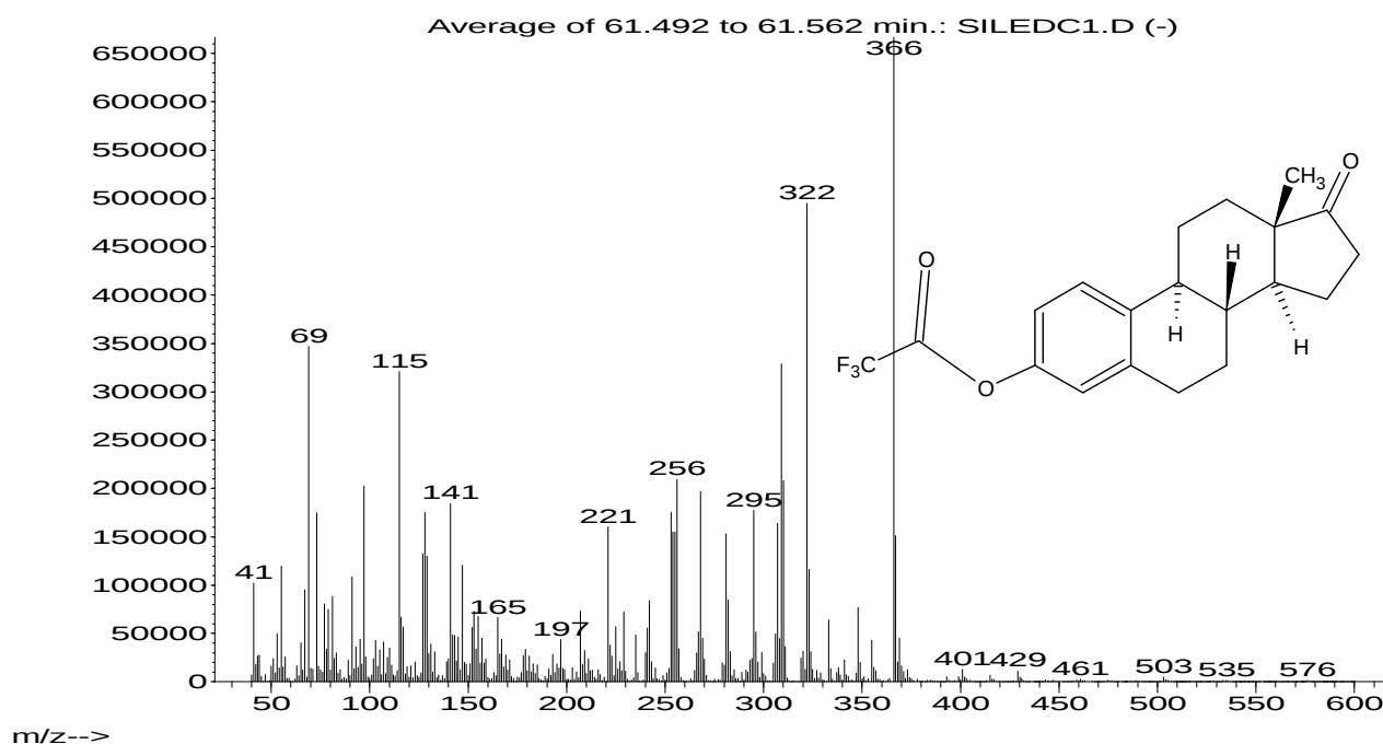
Figure 6.3 Electron impact mass spectrum of the estrone-trifluoroacetate (E1-TFA) derivative. Molecular ion ( M^+ ) m/z 366, ( -CF_3 ) m/z 69.
