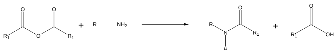
Figure 3.14 Reaction scheme for the reaction of a perfluoroacyl anhydride reagent with a primary amine. R = alkyl or aryl substituent, R 1 = CH 3 , CF 3 , C 2 F 5 or C 3 F 7 [121].
