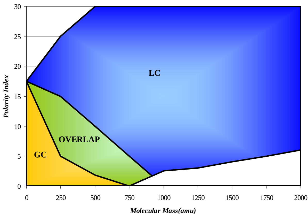
Figure 1.1 Graph showing the analytical domain of GC and LC using polarity versus molecular mass [20]. Copyright Global View Publishing, Pittsburgh, Pennsylvania, U.S.A. Reproduced with permission.
