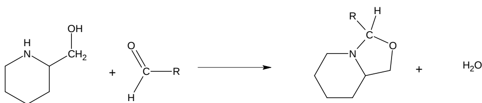
Figure 3.8 Reaction scheme of 2-HMP with an aldehyde [148-151].
