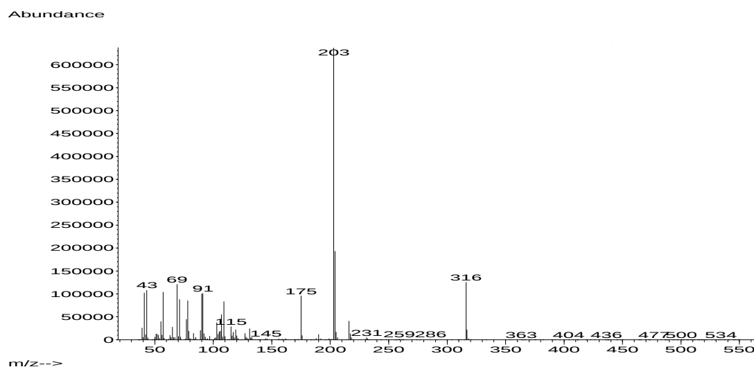
Figure 6.24 Mass spectrum and fragmentation scheme for the main mass spectral fragments obtained for the 4- n -nonylphenol TFA derivative.
