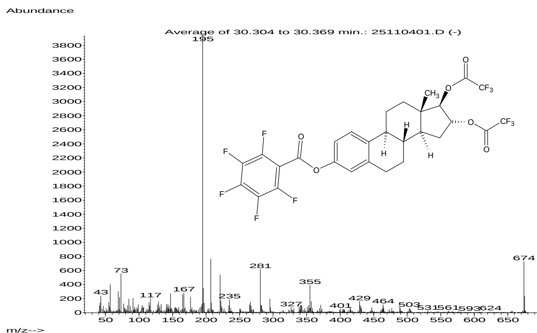
Figure 6.19 The EI Mass Spectrum obtained for the derivative formed from the reaction of 17 \beta -Estradiol (E2) with PFBCl and TFAA. Base peak m/z 195 ( C_7F_5O ), m/z 69 ( CF_3 ) and M^+ m/z 562.
