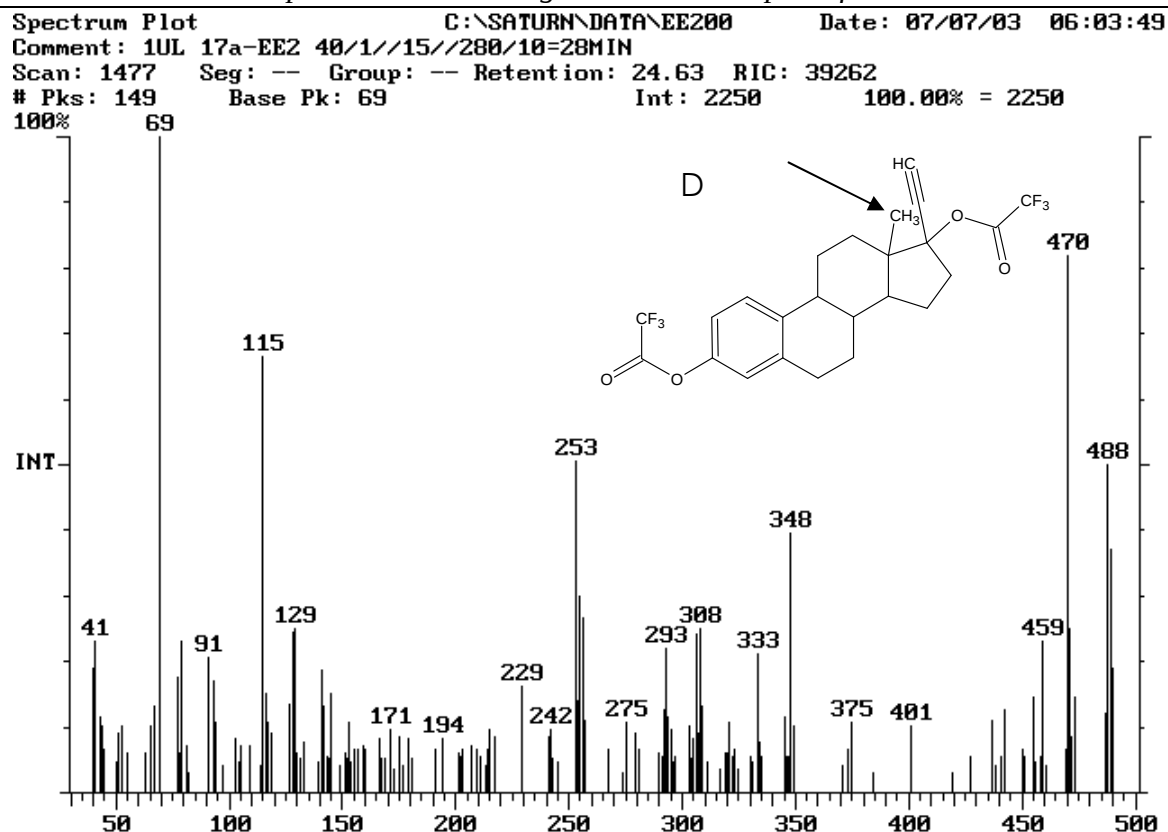
Figure 6.15. The ITD-EI mass spectrum of compound D. The disubstituted EE2-di-TFA derivative.
