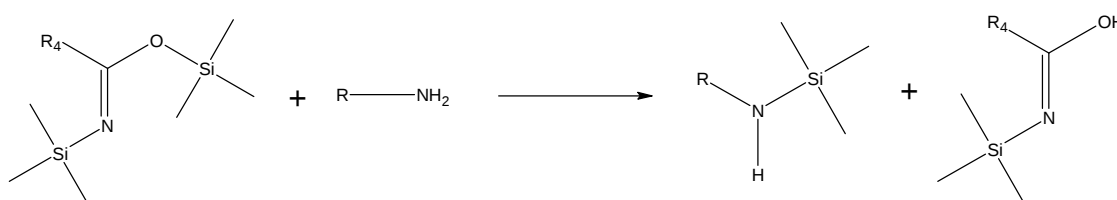
Figure 3.21 Reaction scheme for the reaction of R_4 = \text{CH}_3 (BSA) or \text{CF}_3 (BSTFA) with a primary amine, R = \text{alkyl or aryl substituent} [121].
