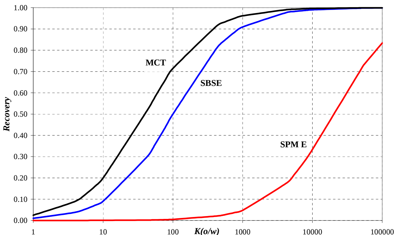
Figure 2.13 Recovery as a function of the octanol-water partition coefficient ( K_{ow} ) of the analyte in 3 different PDMS configurations. The graph was obtained by calculation using equation 2.3 and values for \beta as stated in section 2.5.
