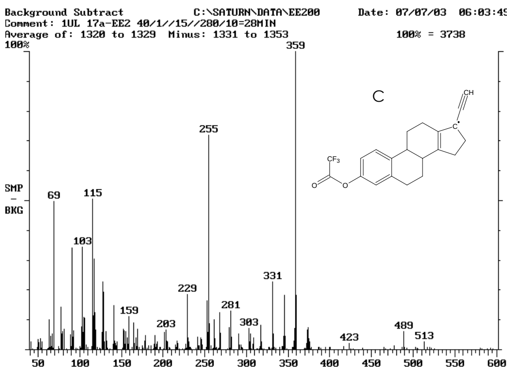
Figure 6.14. The ITD-EI mass spectrum of compound C. The mono-substituted EE2-TFA derivative has undergone a Wagner-Meerwein rearrangement and a water elimination step (dehydration) to form a double bond between the C5 and C6 rings. The methyl group is lost to form base peak m/z 359 and molecular ion at m/z 374.
