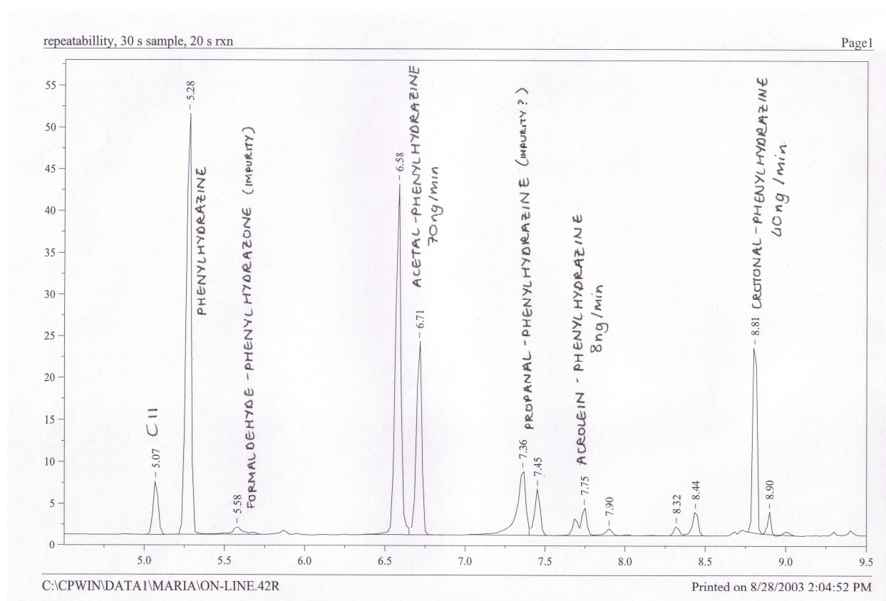
Figure 5.12 The GC-FID chromatogram obtained after desorption of a 100 \mu m PDMS SPME fibre exposed simultaneously for 30 seconds to the permeation gas standards of acetaldehyde, acrolein and crotonal and the phenylhydrazine derivatization reagent. Formaldehyde-phenylhydrazone impurity (5.58 min); Acetal-phenylhydrazone (6.58 & 6.71 min); Propanal-phenylhydrazone (7.36 & 7.45 min); Acrolein-phenylhydrazone (7.68 & 7.75 min) and Crotonal-phenylhydrazone (8.81 & 8.90 min). The double peaks for each derivative, excluding formaldehyde, represent E-Z isomers.
