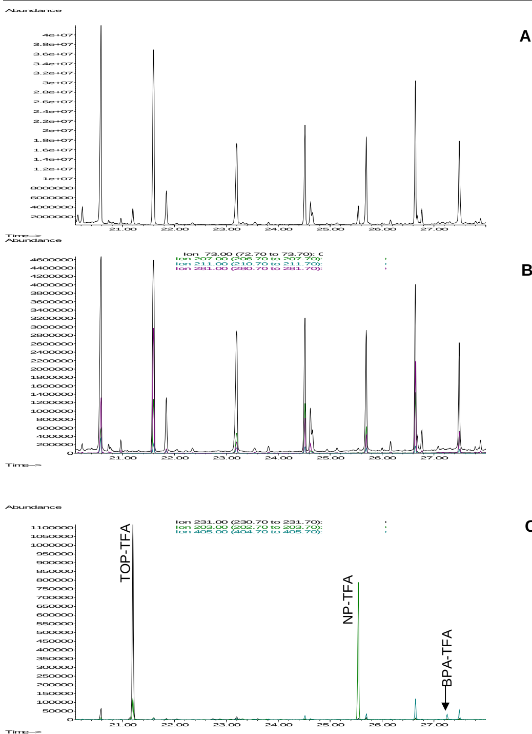
Figure 6.38 (A) Total ion chromatogram of the 20 ml Apies River water sample on PDMS MCT M1. Sample extracted at a flow rate of 50 \mu\text{l}/\text{min} , dried and allowed to react with 5 \mu\text{l} trifluoroacetic acid anhydride for 10 min, followed by thermal desorption.
