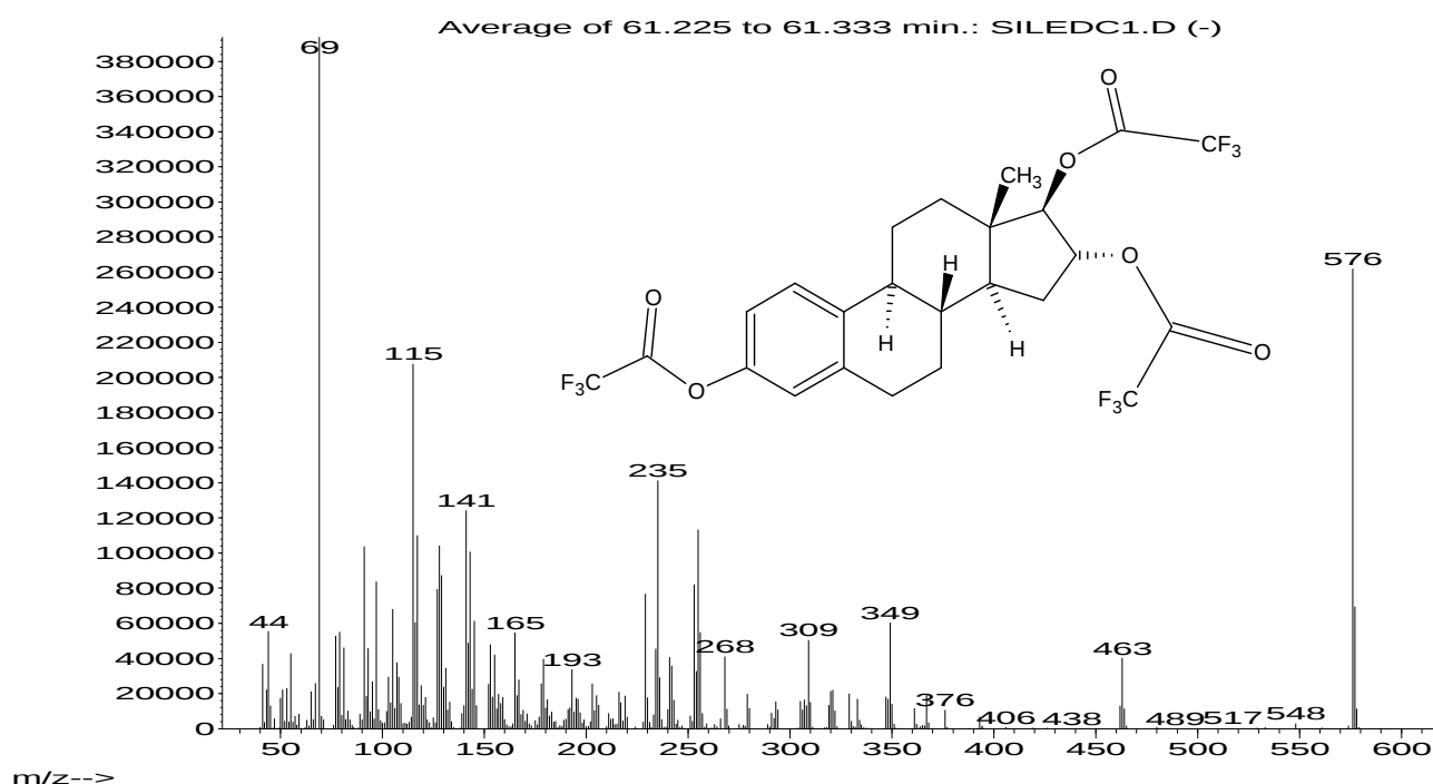
Figure 6.5 Electron impact mass spectrum of the estriol-trifluoroacetate (E3-tri-TFA) derivative. Molecular ion ( M^+ ) m/z 576, ( -CF_3 ) m/z 69.
