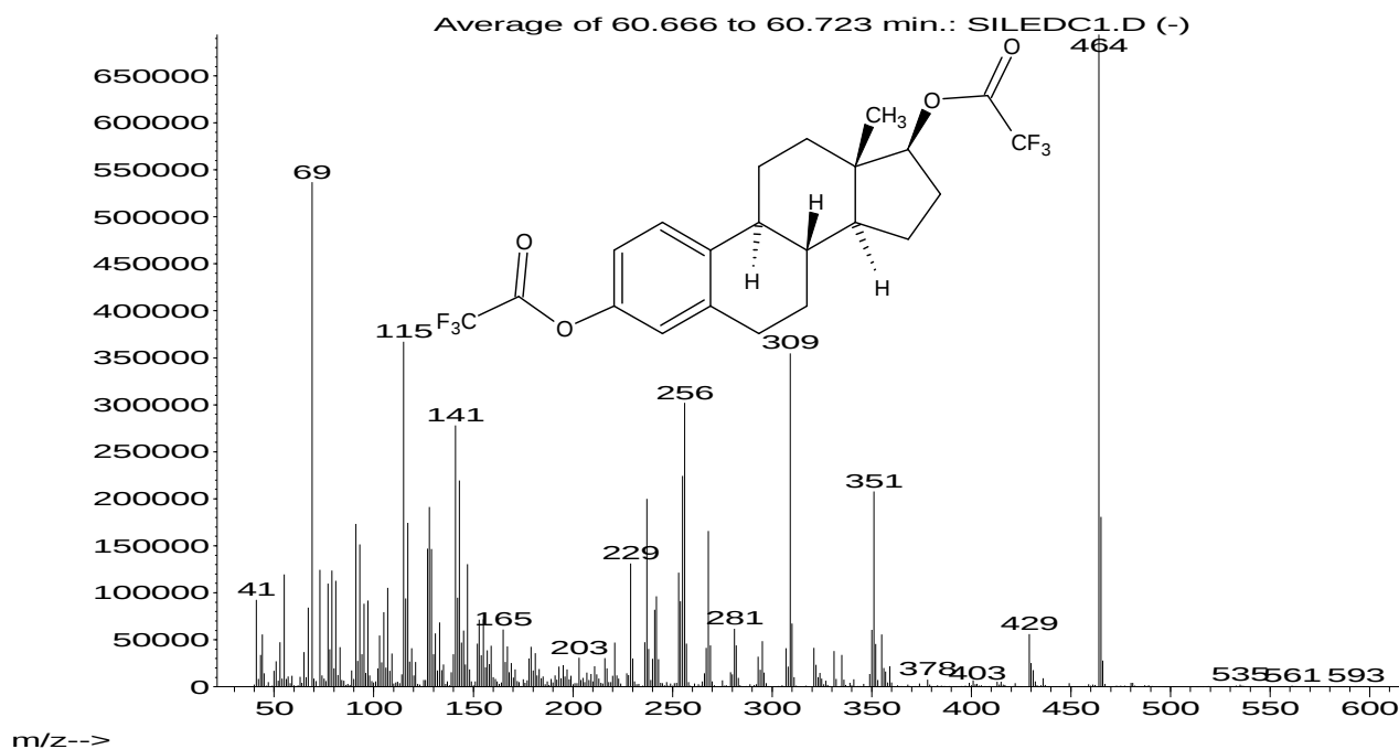
Figure 6.4 Electron impact mass spectrum of the 17β-estradiol-trifluoroacetate (E2-di-TFA) derivative. Molecular ion ( M^+ ) m/z 464, ( -CF_3 ) m/z 69.
