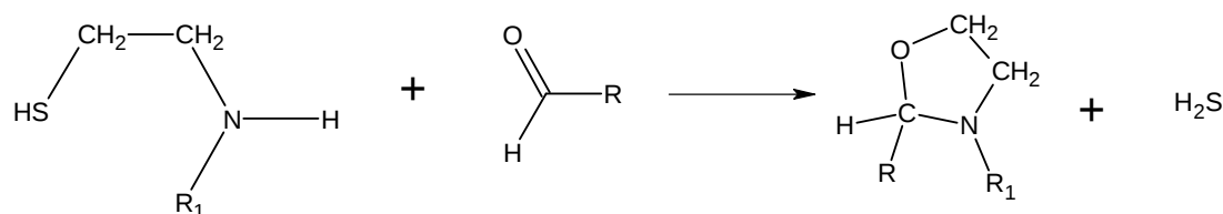
Figure 3.9 Reaction scheme of cysteamine with an aldehyde [136, 152, 153].
