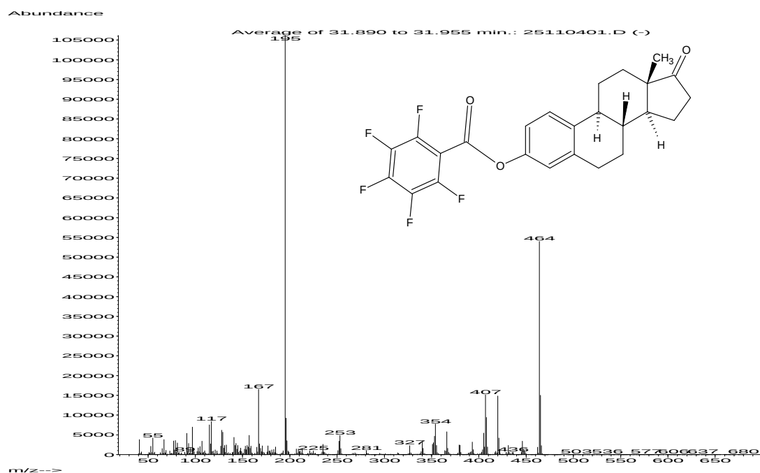
Figure 6.18 The EI mass spectrum obtained for the derivative formed from the reaction of estrone (E1) with PFBCl and TFAA. Base peak m/z 195 ( C_7F_5O ) and M^+ m/z 464.
