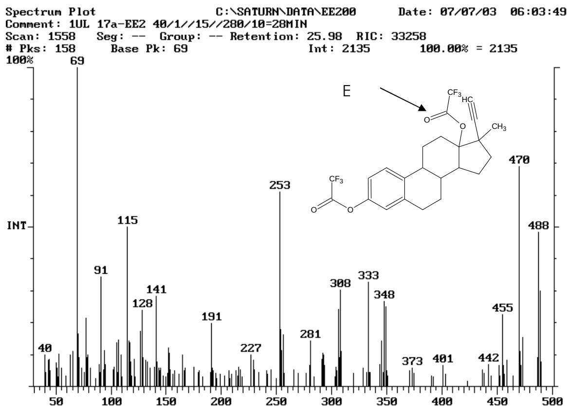
Figure 6.16. The ITD-EI mass spectrum of compound E. The disubstituted EE2-di-TFA derivative after a Wagner Meerwein rearrangement.
