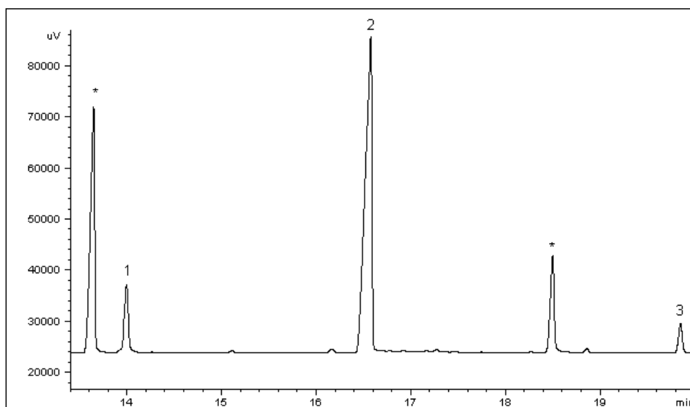
Figure 5.1 Enlarged GC-FID chromatogram obtained by loading PFBHA headspace from the solid reagent into the PDMS MCT. * PDMS thermal degradation peak, 1: Formaldehyde-Oxime, 2: PFBHA, 3: Dodecane (internal standard used to monitor the completeness of desorption of the analytes off the trap. It was added after derivatization using a glass syringe.)
