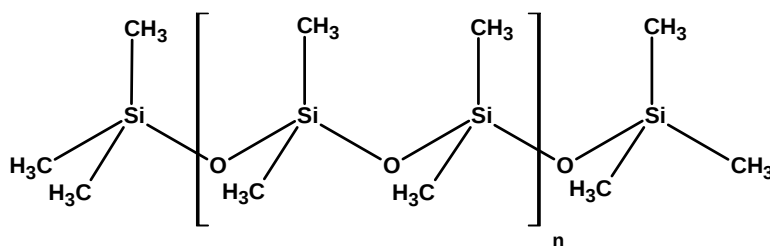
Figure 2.4 The structure of polydimethylsiloxane (PDMS).
