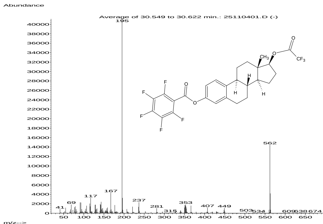
Figure 6.19 The EI Mass Spectrum obtained for the derivative formed from the reaction of 17 \beta -Estradiol (E2) with PFBCl and TFAA. Base peak m/z 195 ( C_7F_5O ), m/z 69 ( CF_3 ) and M^+ m/z 562.
