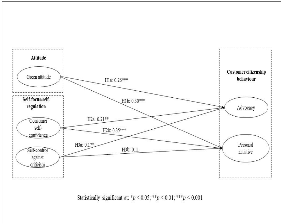
Figure 2: Structural model
