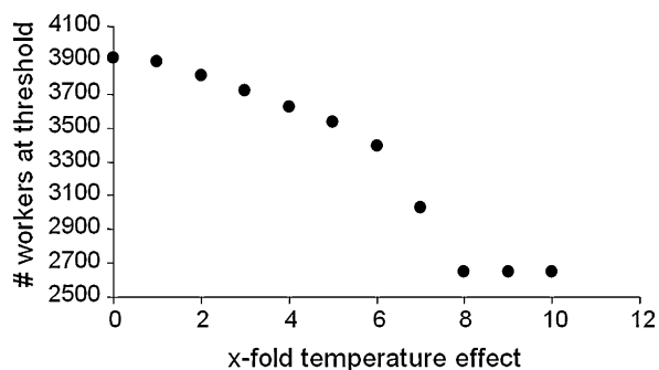
Fig. 7. Survival thresholds (i.e. minimal number of initial bees needed for colony survival) in the model in relation to the temperature effect (0: no temperature effect, 1: empirical temperature effect, >1: accordingly magnified temperature effect) (TEMP.GRAIDENT = 0.45, MAX.HEATEDCELLS.PER.BEE = 2.65).
