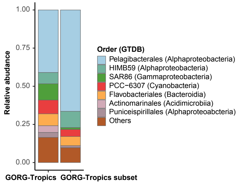
Fig. S1. Taxonomic composition of SAGs selected for this study, compared to the entire GORG-Tropics dataset.
