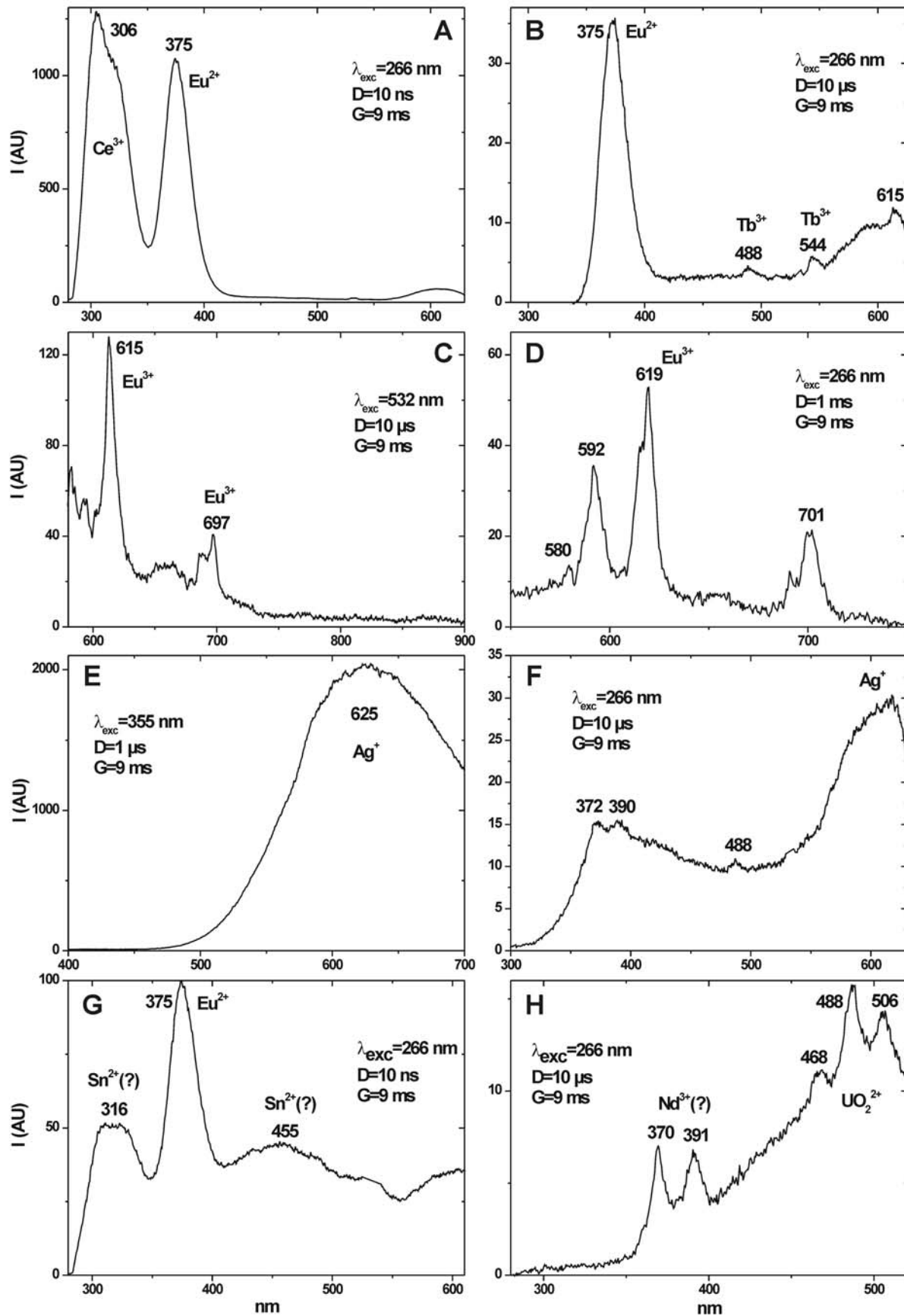
Fig. 4. Time-resolved luminescence spectra of endogenic barite from the Kremikovtsi deposit demonstrating different emission bands: (A) \text{Ce}^{3+} , \text{Eu}^{2+} ; (B) \text{Eu}^{2+} , \text{Tb}^{3+} ; (C) \text{Eu}^{3+} ; (D) \text{Eu}^{3+} ; (E) \text{Ag}^+ (F) \text{Ag}^+ (G) \text{Eu}^{2+} , \text{Sn}^{2+} ; (H) \text{Nd}^{3+} , \text{UO}_2^{2+} .
