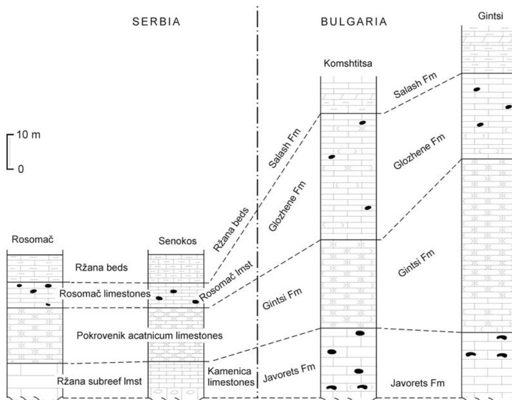
Fig. 4. Simplified columnar sections of the Middle Callovian–Upper Jurassic sediments of the Infra-Getic domain in the Piroč-Godeč area. Legend as for Fig. 3.
