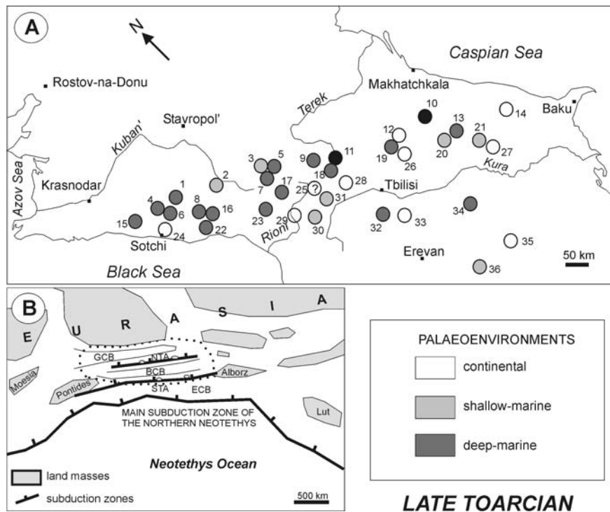
Fig. 4. The Late Toarcian palaeoenvironments (A) and the palaeogeographic outline (B) of the Caucasus (explanation of "zones" – Fig. 3A). "?" marks uncertainty in the interpretation of the continental palaeoenvironments, because of the doubtful establishment of hiatus. GCB, Greater Caucasus Basin, BCB, Black Sea – Caspian Sea Basin, ECB, Exterior Caucasian Basin, NTA, Northern Transcaucasian Arc, STA, Southern Transcaucasian Arc. The dotted line bounds the Caucasian Sea.
