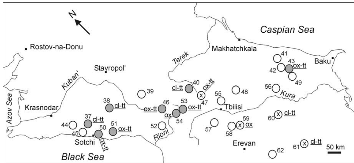
Fig. 7. The location of the Callovian-Tithonian carbonate buildups in the “zones” of the Caucasus (data was extracted from ROSTOVITSEV et al. (1992); for the western part of the Caucasus, it was supported by personal field observations) (for an explanation of the “zones”, see Fig. 3B). “Zones” where carbonate buildups were evidently documents are highlighted as gray, while “zones” where only coral founds are known are marked by x. The age of buildup- or coral-bearing deposits is indicated.
