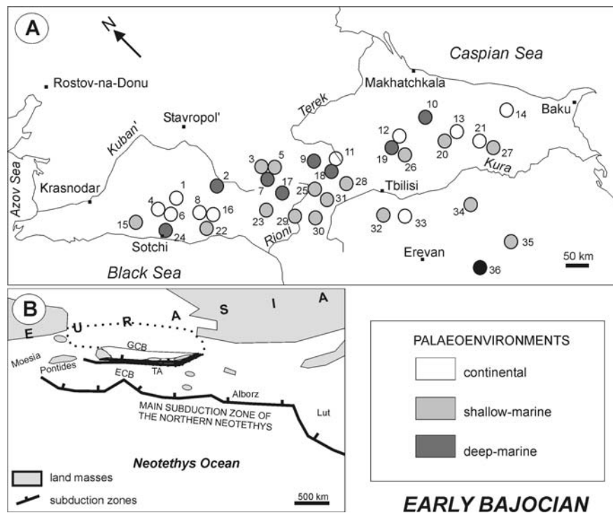
Fig. 5. The Early Bajocian palaeoenvironments (A) and the palaeogeographic outline (B) of the Caucasus (explanation of “zones” – Fig. 3A). GCB, Greater Caucasus Basin; ECB, Exterior Caucasian Basin; TA, Transcaucasian Arc. The dotted line bounds the Caucasian Sea.
