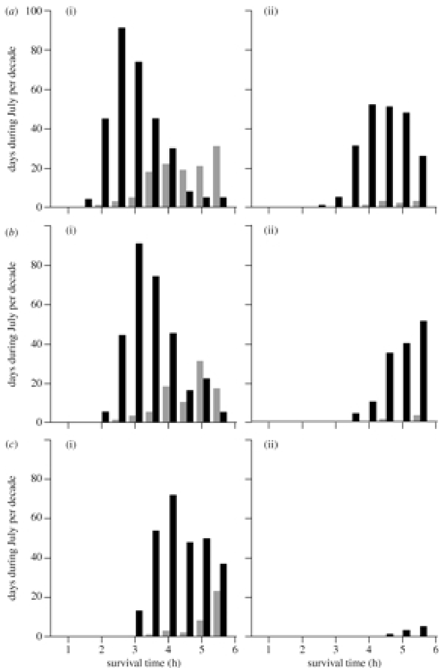
Figure 2. Small birds at Yuma AZ, U.S.A. will be exposed to survival times < 6 hr much more frequently during mid-summer in the 2080s compared to the 1990s. Survival time distributions are shown for three body mass ( M_b ) values (5 g, 25 g and 50 g), and dehydration tolerances equivalent to 11% of M_b (left-hand graphs) and 22% of M_b (right-hand graphs). Survival time distributions were modeled using daily maximum air temperature ( T_a ) data for the hottest month (July) during the 1990s, and the predicted increase in maximum T_a for this location (IPCC 2007).
