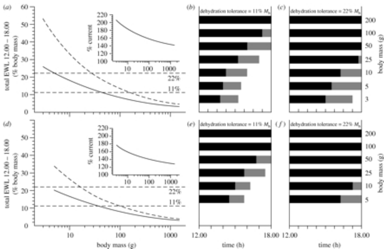
Figure 1. Predicted increases in air temperature ( T_a ) maxima for Yuma AZ, USA (upper graphs) and Birdsville, Australia (lower graphs) will cause large increases in evaporative water requirements (left graphs), and substantially decreased survival times (right graphs). Evaporative water requirements and survival times are modeled for birds resting in the shade between 12:00 and 18:00. The inset graphs show water requirements predicted for the 2080s as percentages of current values. In the right hand graphs, the x-axes correspond to the period 12:00 – 18:00, with the horizontal bars indicating the time (to the nearest 15 min) at which evaporative water losses exceed dehydration tolerance values [11 or 22 % of body mass ( M_b ), indicated by horizontal dashed lines in left-hand graphs]. The M_b minima are 3 g for Yuma (corresponding to small hummingbirds, e.g. Selasphorus spp.) and 5 g for Birdsville (thornbills, Acanthiza spp.).
