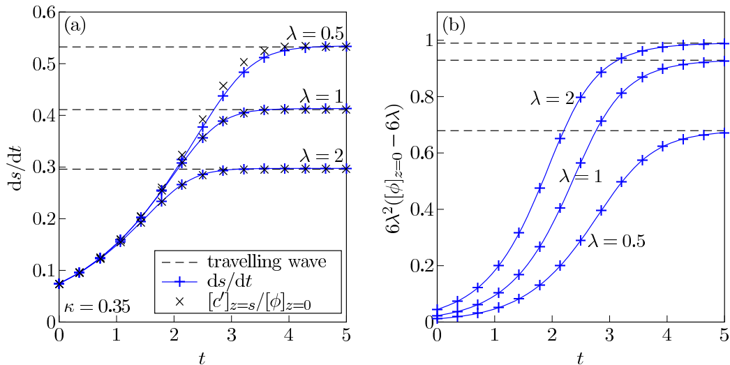
Figure 4: Time-dependent 1D numerical solutions for varying \lambda : (a) biofilm surface velocity s_t , (b) basal EPS volume fraction \phi|_{z=0} .
