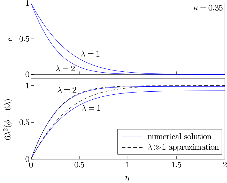
Figure 2: Numerical solutions for c and \phi using (??) 2 and (??), with \Lambda given by (??). Results for \phi are plotted as 6\lambda^2(\phi - 6\lambda) for ease of comparison with the large \lambda approximate solutions (??) (shown dashed).
