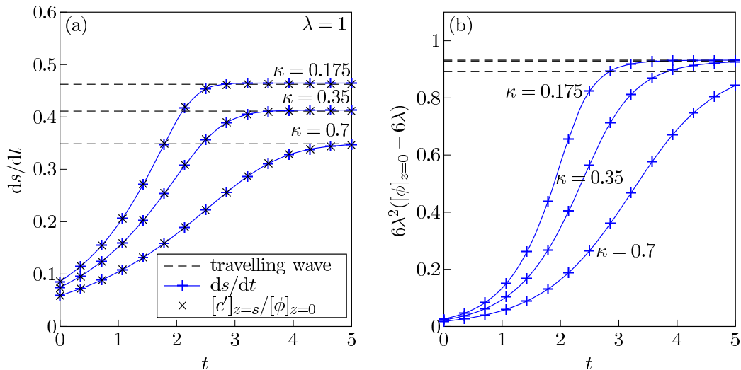
Figure 5: Time-dependent 1D numerical solutions for varying \kappa : (a) biofilm surface velocity s_t , (b) basal EPS volume fraction \phi|_{z=0} .
