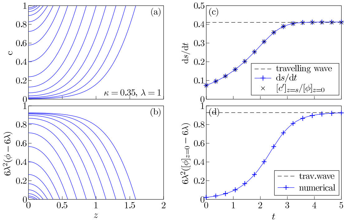
Figure 3: Time-dependent 1D numerical solution for \lambda = 1 , \kappa = 0.35 : (a) nutrient profiles c , (b) EPS volume fraction profiles \phi , (c) biofilm surface velocity s_t , (d) basal EPS volume fraction \phi|_{z=0} . Data for \phi are plotted as 6\lambda^2(\phi - 6\lambda) .
