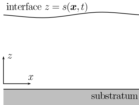
Figure 1: Geometry of the biofilm. A bacterial layer grows upwards from a wall at z = 0 , and is bounded by its surface at z = s .
