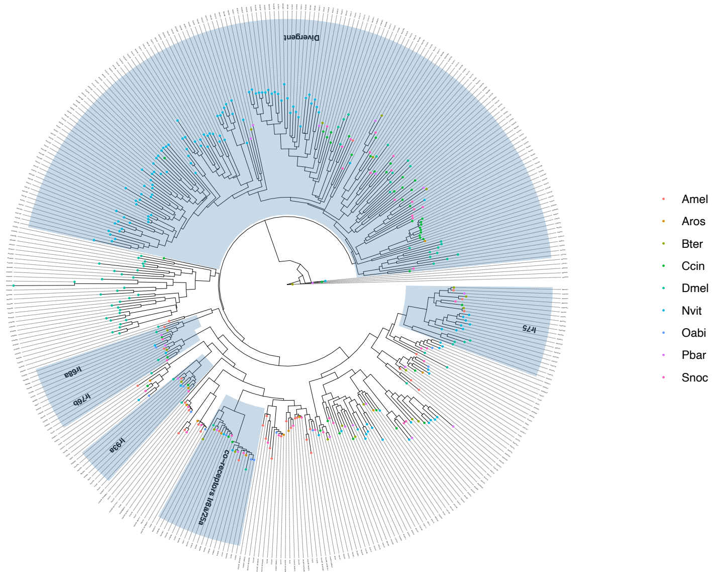
Supplementary Figure 5: Phylogenetic tree of IR genes from Sirex noctilio (Snoc), Apis mellifera (Amel), Athalia rosae (Aros), Bombus terrestris (Bter), Cephus cinctus (Ccin), Drosophila melanogaster (Dmel), Nasonia vitripennis (Nvit), Orussus abietinus (Oabi) and Pogonomyrmex barbatus (Pbar). Sub-families of interest are highlighted and include: Divergent receptors and Co-receptors (Ir8a and Ir25a).
