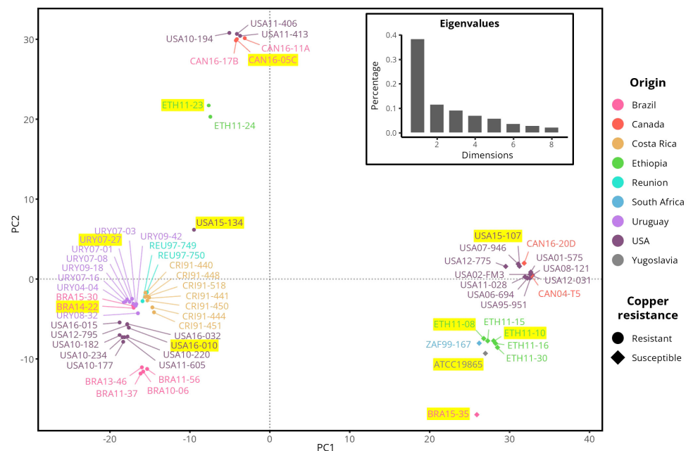
Fig. 1. Principal component analysis of Xanthomonas hortorum pv. gardneri strains based on the presence/absence of accessory genes. PC1 contained more than three times the variation of PC2. PC1 separates strains containing the L-plasmid (PC1 coordinates < 0) from strains lacking the L-plasmid (PC1 coordinates > 0). Strains are colored by country, and the labels of strains that were experimentally tested for copper tolerance are highlighted in yellow (Supplementary Table S6). JS749-3 and strains from Uruguay were also reported as copper tolerant (Montelongo García 2012; Richard et al. 2017a).
