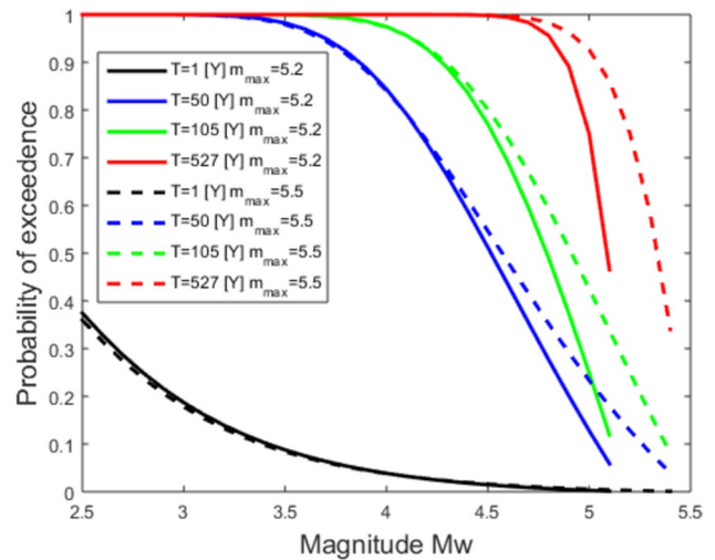
Fig. 2 Probability of exceeding a given magnitude within 1, 50, 105, and 527 years
