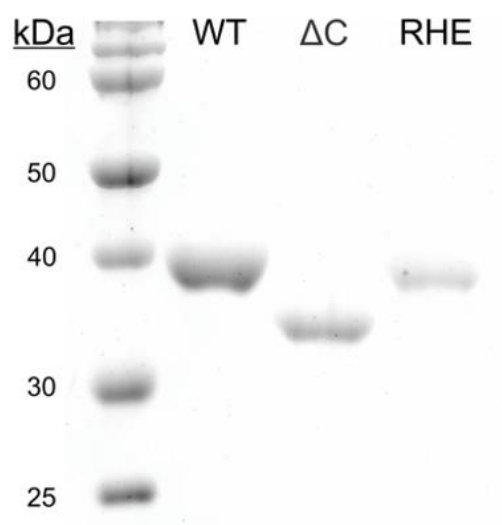
Figure A3.1: Coomassie stained SDS-polyacrylamide gel with 100 \mu g loaded each of PfPdx1 wildtype (WT), the C-terminal truncated form of PfPdx1 ( \Delta C) and the PfPdx1 RHE mutant. PfPdx1 - \Delta C was shown to be \sim 35 kDa compared to the wild-type (WT) PfPdx1 at 37.5 kDa, confirming the 31 amino acid deletion.
