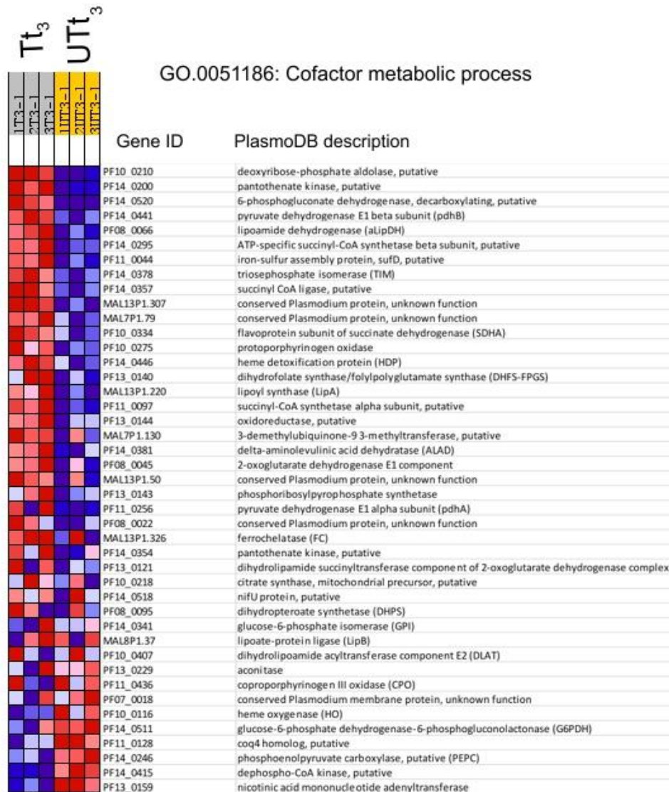
Figure 4.9: GSEA analysis of Tt 3 vs. UTt 3 . Heat maps of gene sets found to be enriched in GSEA. GSEA was calculated with P \leq 0.05 and had a false discovery rate (FDR) \leq 0.25 (25%). Red indicates increased transcript expression levels in the respective arrays, whereas blue indicates decreased transcript expression.
