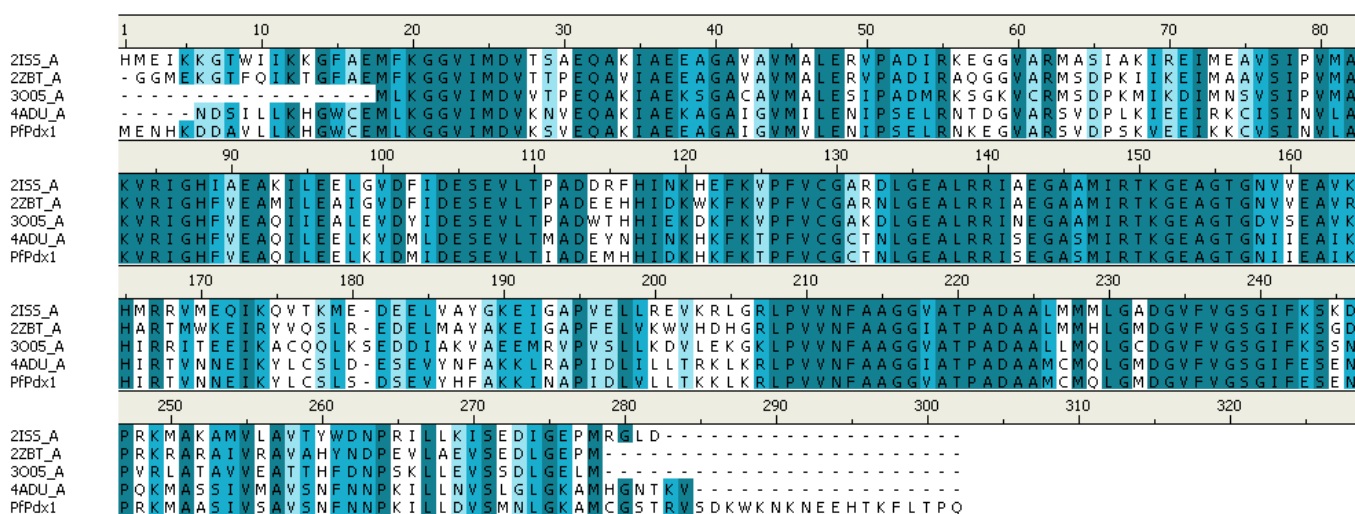
Figure 2.4: Multiple protein sequence alignment (MSA) generated for Pdx1 homologues. Aligned crystal structures of T. maritima (2ISS), T. thermophilus (2ZBT), P. berghei (4ADU), S. cerevisiae Pdx1 (3005) and Pf Pdx1 (pyridoxine biosynthetic enzyme pdx1 homologue, NCBI reference sequence XP_966196.1). Conserved residues indicated in dark blue, with residues with similar properties indicated in light blue.
