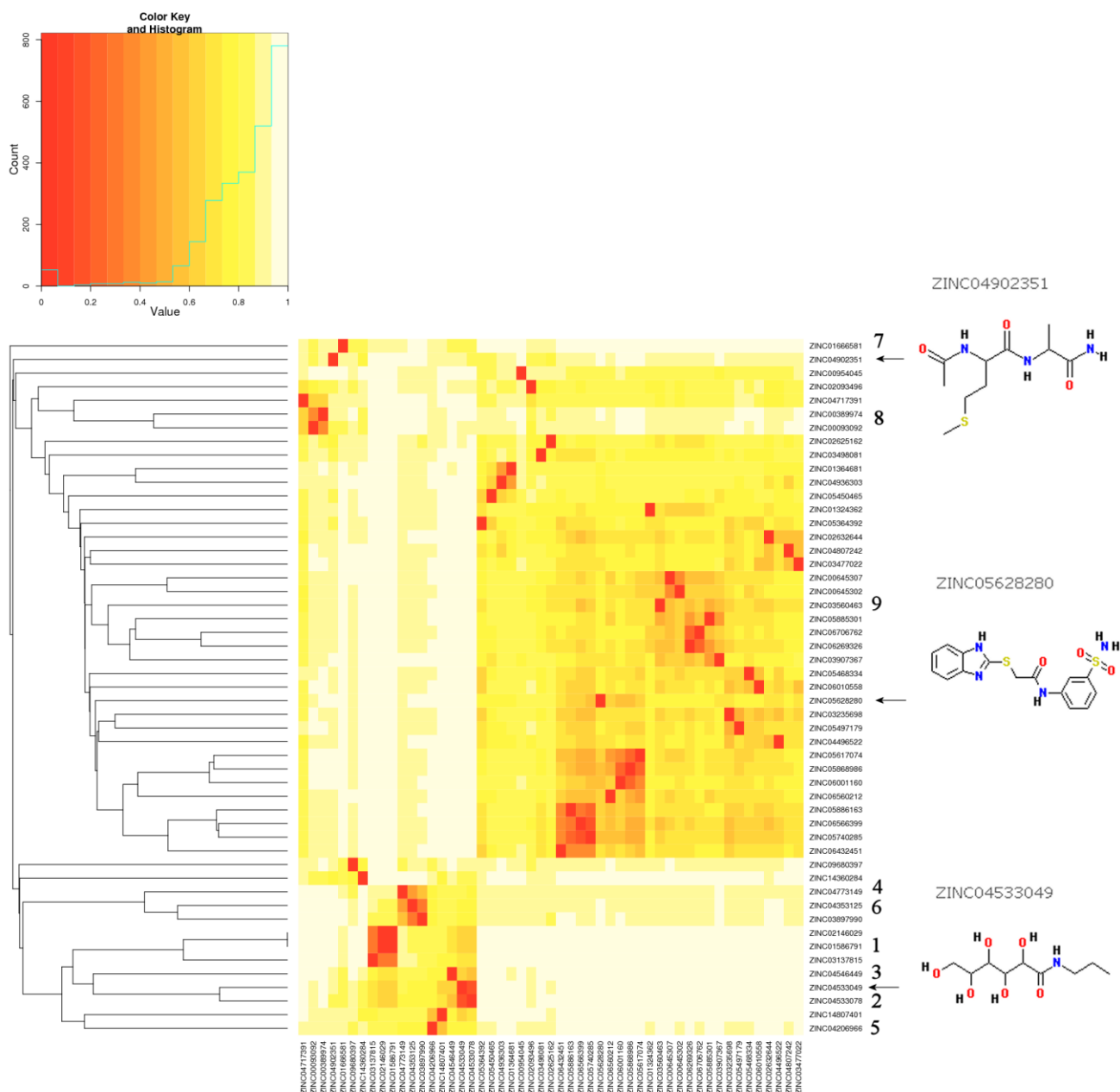
Figure 2.19: Structural pairwise similarity clustering of the best 50 pharmacophore-identified ligands by chemical similarity. Similar ligands are indicated in shades of red, in which the most intense red represents a high degree of chemical similarity or compound identity. Numerical values next to the ligand names, on the right side of the figure, represent the best-scoring in which 1 represent the best scoring ZINC01586791 ligand. The heat map was generated using Chemmine ( http://chemmine.ucr.edu ).
