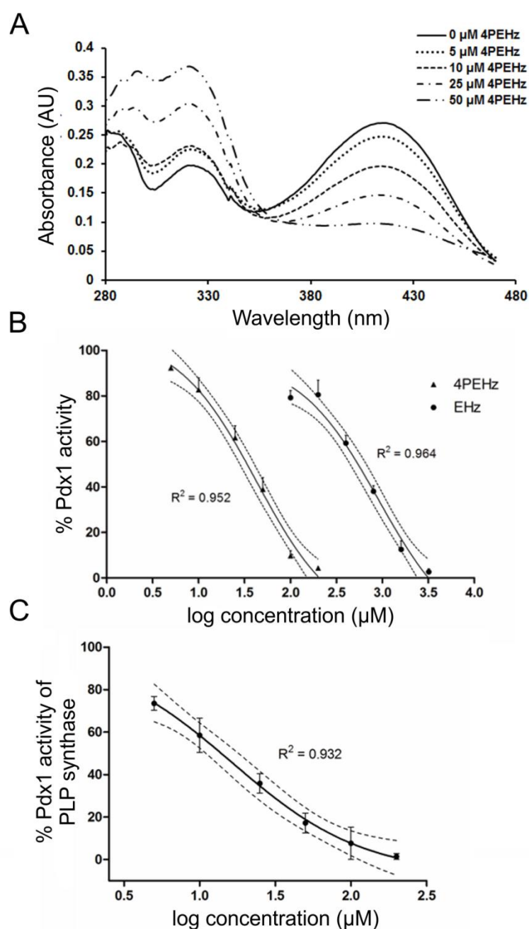
Figure 3.7: E4P analogues and their effect on PfPdx1 . A) Incubation of PfPdx1 (200 \mu g) with increasing concentrations of 4PEHz and measured PLP production visible at 414 nm. Results shown represent a single observation from independent triplicate experiments. B) Dose-response curves of 4PEHz and EHz inhibition on PfPdx1 (200 \mu g). Results were generated from three independently performed experiments, performed in duplicate, with the SEM indicated. The 95% CI is shown as dotted lines. C) Effect of 4PEHz on oligomeric PfPdx1 and PfPdx2 . Reaction conditions included 100 \mu g of each PfPdx1 and PfPdx2 with 0.5 mM R5P, G3P and 20 mM L-glutamine as only nitrogen source. Results were generated from three independent experiments performed in duplicate, with the SEM indicated. The 95% CI is given in dotted lines.
