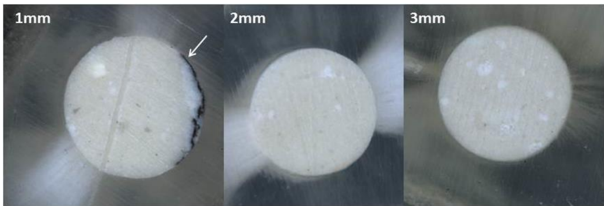
Figure 4.6: Stereomicroscopic view of transverse sections of a representative specimen of the MTA Plus™ group. Note that leakage is visible in this specimen only at the 1 mm level (arrow).
