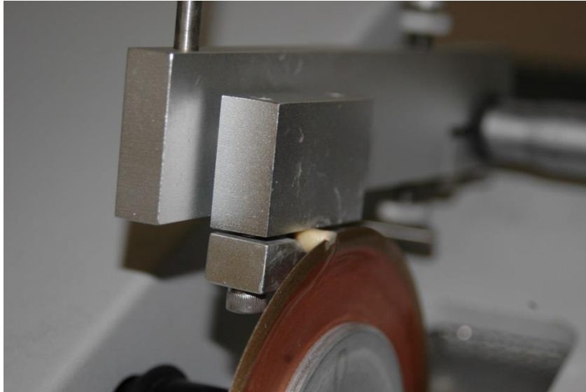
Figure 3.27: Specimens sectioned transversely with a wafering blade in 1 mm increments.
