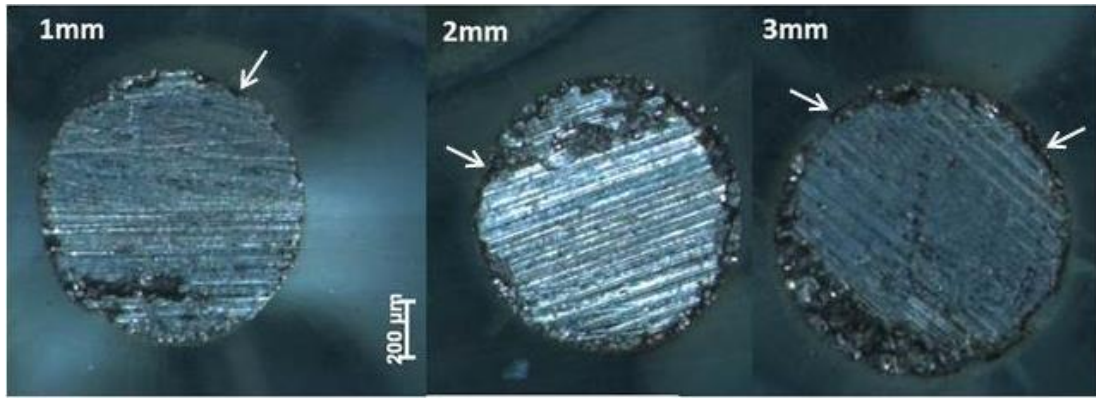
Figure 4.11: Stereomicroscopic view of transverse sections of a representative specimen of the Permited Amalgam group. Note the extensive leakage up to the 3 mm level (arrows).
