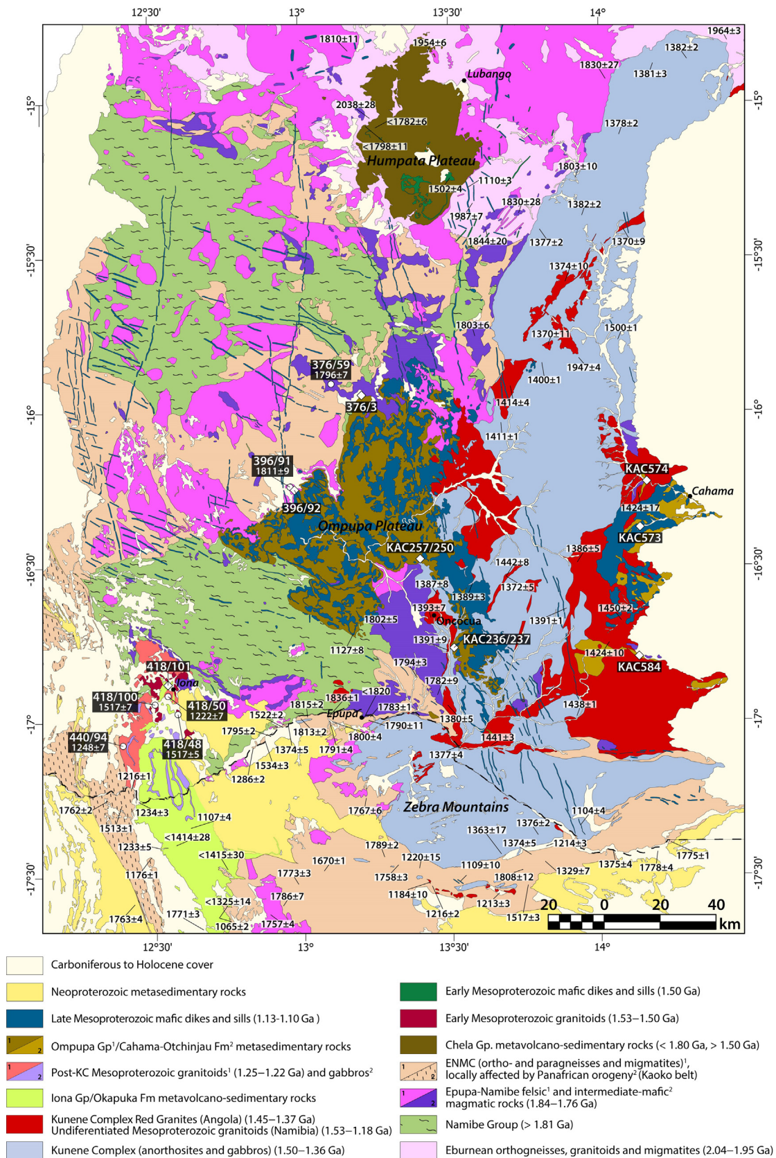
Fig. 2. New geological map for the study area based on the map of the Geological Survey of Namibia 1:250,000 and Kröner et al. (2010) for Namibia, and on the UTE-1 geological map at 1:500,000 scale of the Geological Institute of Angola (Rodrigues et al., 2021a). References for the reported published crystallization ages are the same as for Fig. 1.
