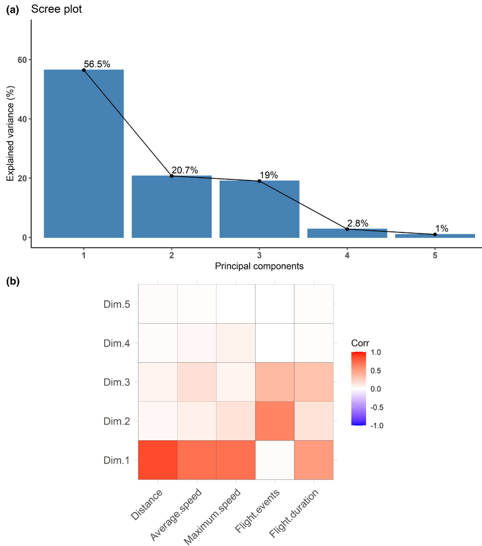
FIGURE 1 Scree plot (a) and correlation plot (b) from a principal component analysis on flight-related traits in three tephritid species. The scree plot indicates how much variance is explained by each principal component. The correlation plot indicates how each trait of interest is correlated with each dimension (principal component). The darkest of red indicates a strong positive correlation, and the darkest shade of purple indicates a strong negative correlation. A white square indicates an absence of correlation between a given trait and principal component.
