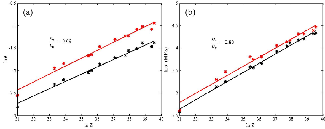
Figure 6.6: Plots of (a) \ln \varepsilon against \ln Z and (b) \ln \sigma against \ln Z indicating how the relationship between \varepsilon_c and \varepsilon_p (left) and between \sigma_c and \sigma_p (right) were found for AISI 321 stainless steel.
