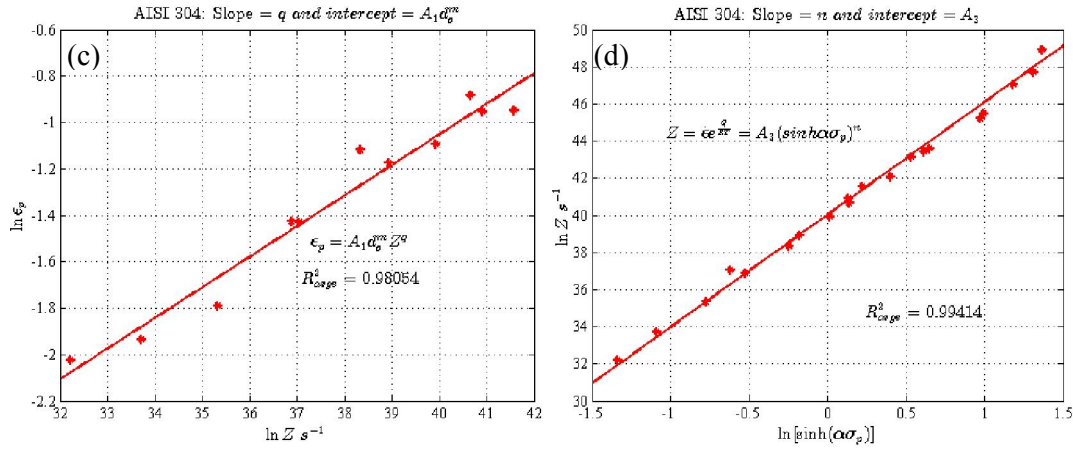
Figure 6.8: Plots used for the determination of n , (A_1 d_o^m) and A_3 values for AISI 304 steel
