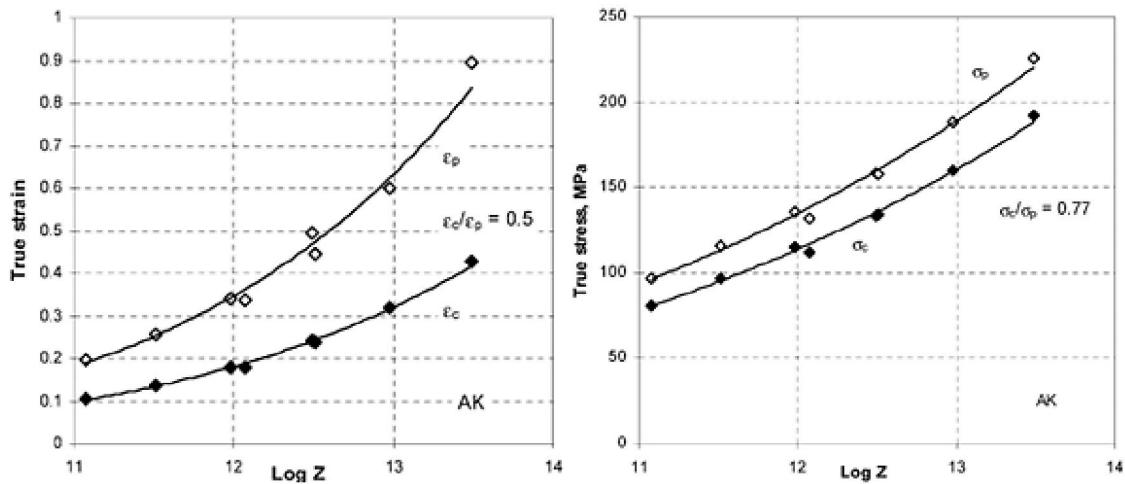
Figure 3.4: Plots indicating how to find the critical stress \sigma_c and the critical strain \varepsilon_c [34].
