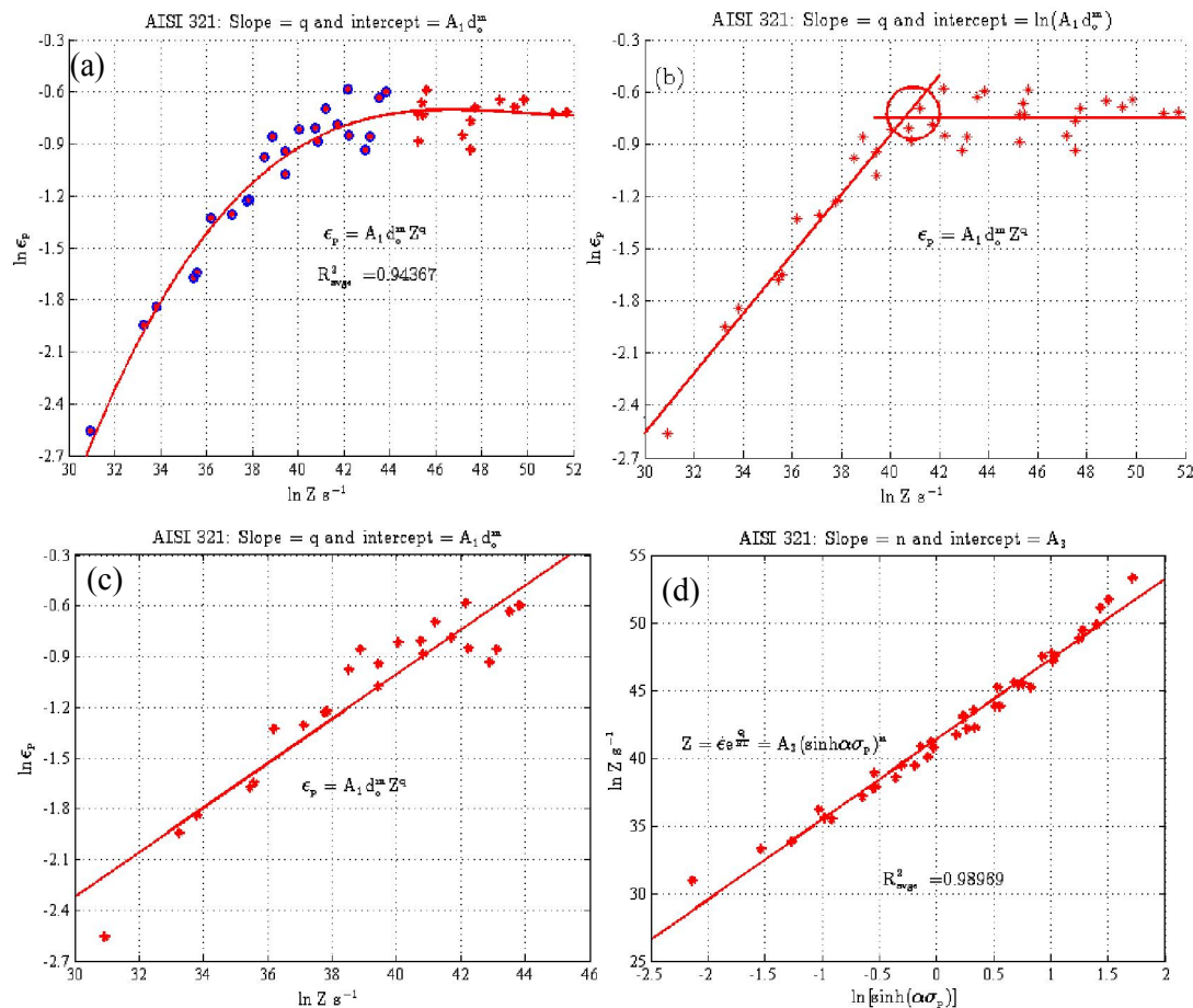
Figure 6.2: Plots used for the determination of n , (A_1 d_o^m) and A_3 values for AISI 321 steel
