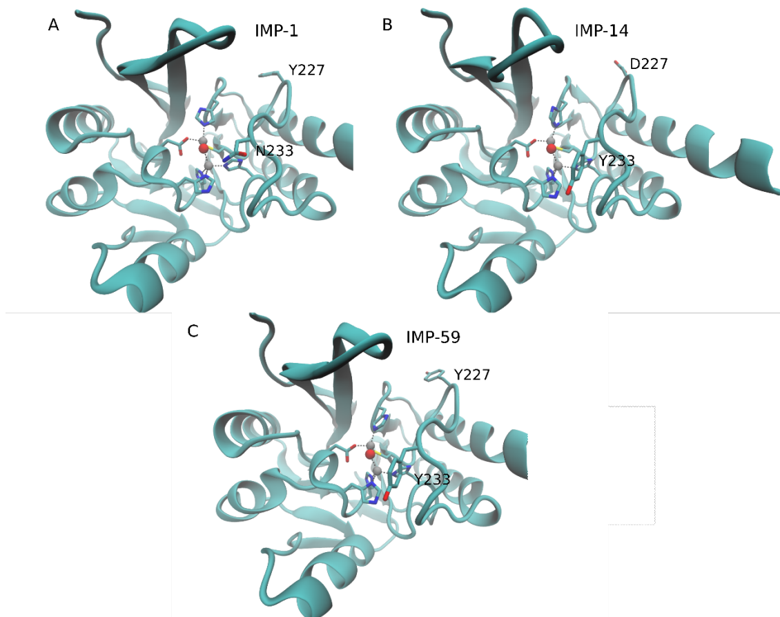
Figure S1. Comparison of the structures of the IMP variants showing the mutations in the L10 loop. IMP-1 (A), IMP-14 (B) and IMP-59 (C)
