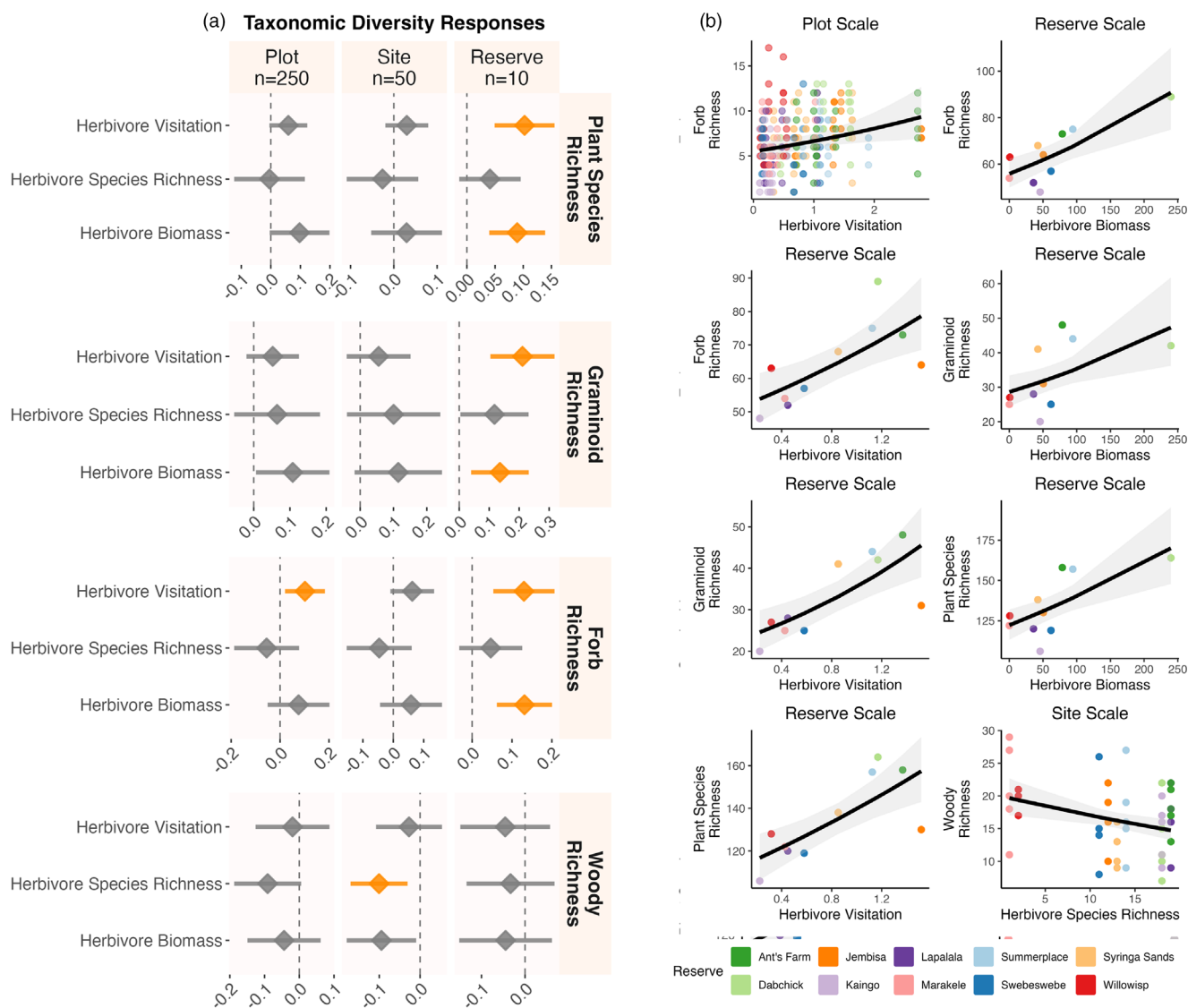
FIGURE 2 Relationships between plant taxonomic diversity and herbivore regime. (a) Panels showing model effect sizes for how the herbivore regime is linked to total, graminoid, forb and woody species richness at the plot, site and reserve scales. The error bars represent the 95% confidence interval and the colour indicates whether the variable has a significant effect (after Bonferroni correction); grey = non-significant, orange = significant. (b) Significant (after Bonferroni correction) bivariate relationships between plant taxonomic diversity and herbivore variables, showing both the data (points) and model predictions (lines). The grey ribbons represent the 95% confidence interval. Herbivore biomass is given in kg/ha and herbivore visitation represents the number of independent detections per day.
