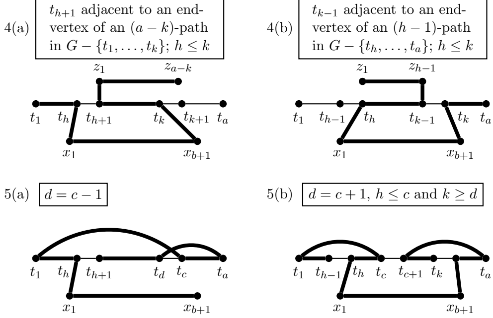
Figure 3. Illustrations of indirect proofs of Lemma 2.3(4(a)–(b)) and 2.3(5(a)–(b)). In each case, the heavy lines indicate a path of order greater than a + b that would be in G if a condition in the corresponding item was violated.
