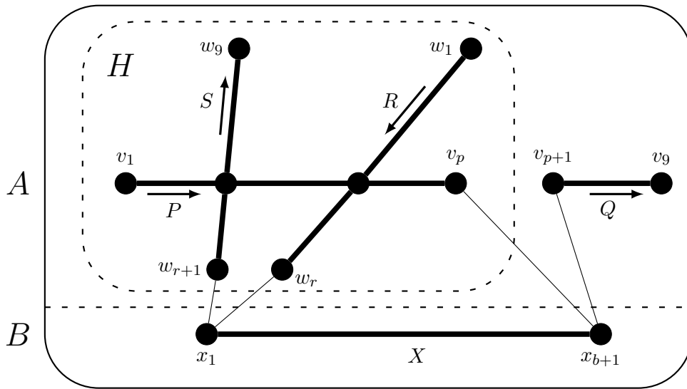
Figure 5. Illustrating a problematic configuration (X, P, Q, R, S) and the associated problematic component H , as defined in Definition 3.1, for the case p \geq r . Note that Q may be in H and each of R and S may intersect P and Q in several vertices.
