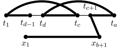
Figure 4. Illustrations of indirect proofs of Lemma 2.3 (5(c)–(e)). In each case, the heavy lines indicate a path of order greater than a + b that would be in G if a condition in the corresponding item was violated.
