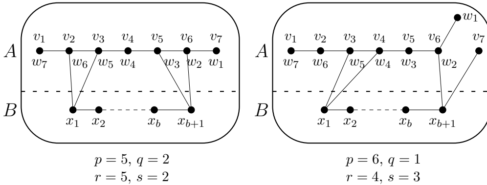
Figure 1. The two problematic configurations for a = 7 .
