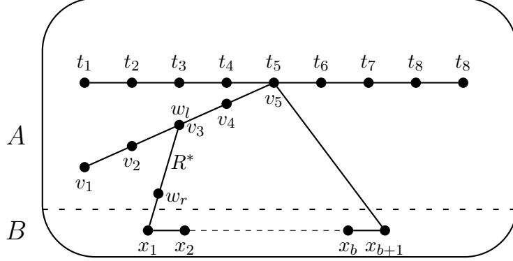
Figure 7. A step in the proof of Lemma 3.8 (A2.1).
