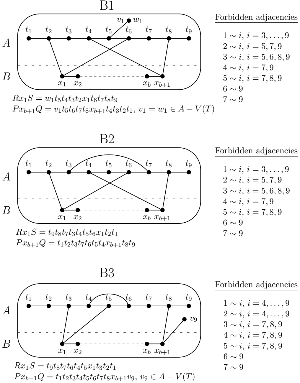
Figure 9. Configurations of Type B, consisting of (X, P, Q, R, S, T) = \langle E(X) \cup E(Rx_1S) \cup E(Px_{b+1}Q) \cup E(T) \rangle .
