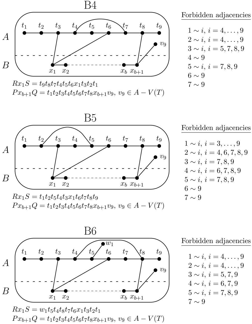
Figure 10. Configurations of Type B, consisting of (X, P, Q, R, S, T) = \langle E(X) \cup E(Rx_1S) \cup E(Px_{b+1}Q) \cup E(T) \rangle — continued.
