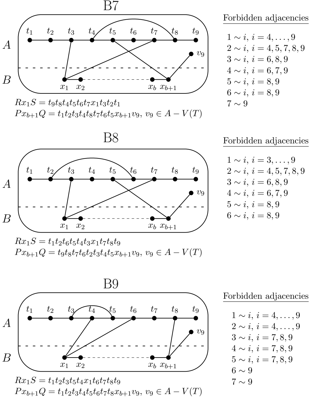
Figure 11. Configurations of Type B, consisting of (X, P, Q, R, S, T) = \langle E(X) \cup E(Rx_1S) \cup E(Px_{b+1}Q) \cup E(T) \rangle — continued.
