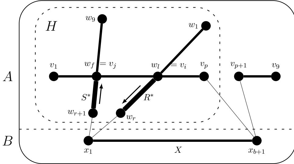
Figure 6. Illustrating the subpaths R^* and S^* in a problematic configuration (X, P, Q, R, S) with p \geq r .
