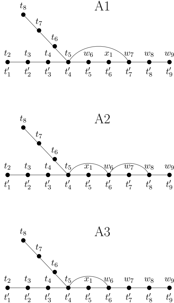
Figure 15. The path T' when step 3(b) is applied to type A-configurations.
