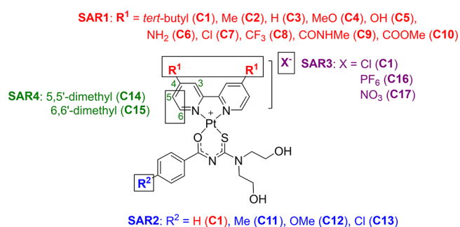
Figure 1. Mixed-ligand platinum(II) complexes showing the four SAR sites and their respective substituents.
