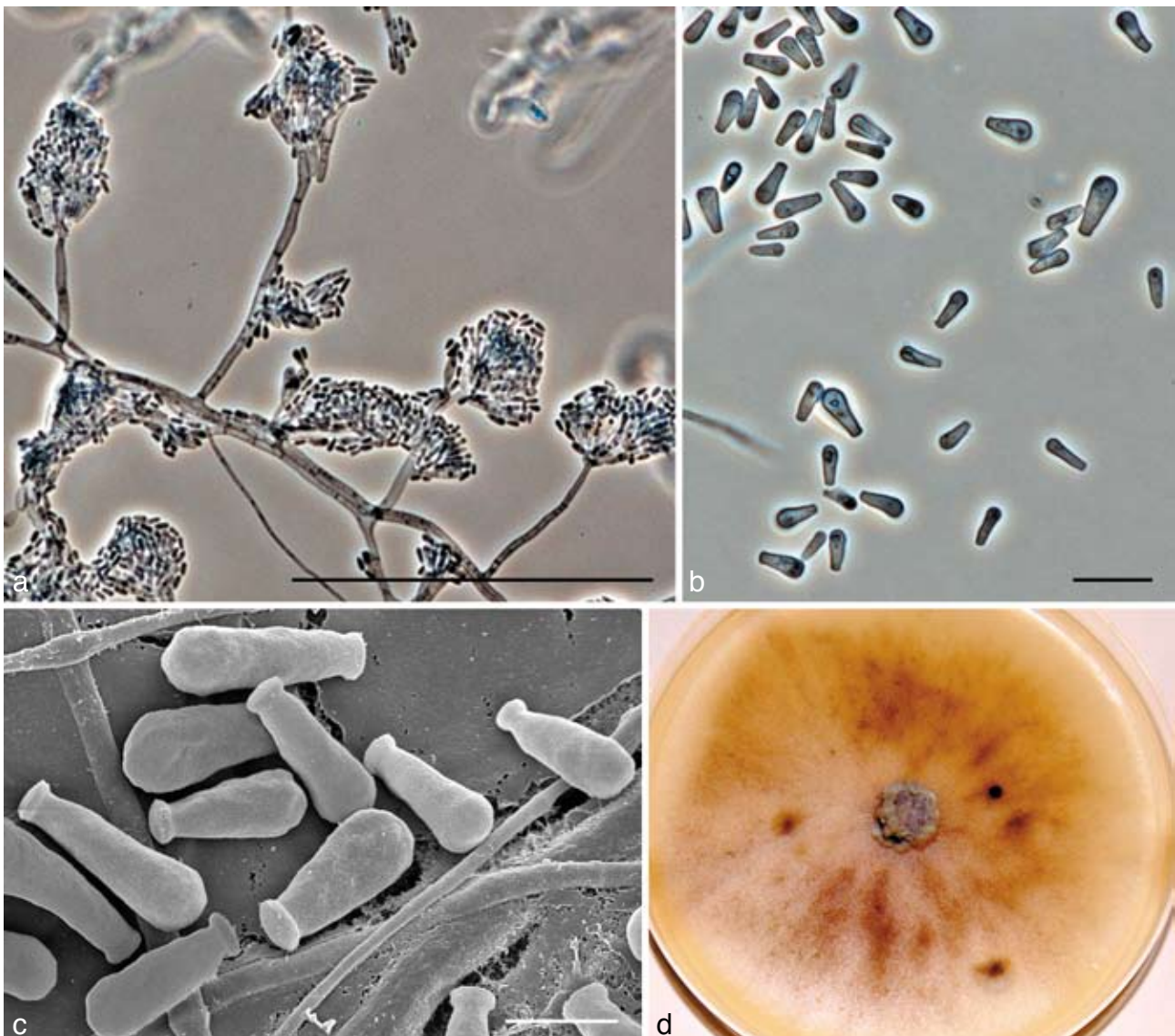
Fig. 7 Morphological characters of anamorph structures of Ophiostoma tapionis sp. nov. a. Hyalorhinocliadiella anamorph; b. conidia; c. SEM of conidia; d. fourteen day old culture on MEA. — Scale bars: a = 100 \mu\text{m} ; b = 10 \mu\text{m} ; c = 3 \mu\text{m} .
