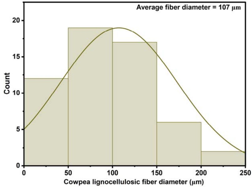
Figure 1: Histogram showing the diameter size distribution of cowpea lignocellulosic fibers.
