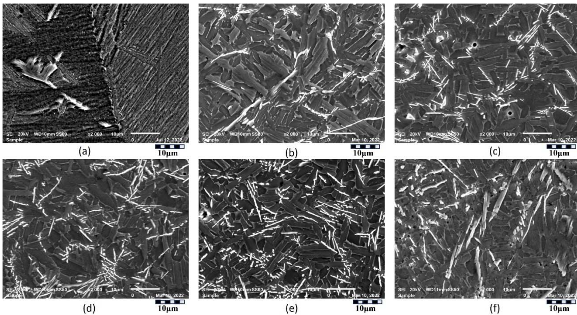
Figure 10: SEM micrographs of the TiB/Ti6Al4V samples at various TiB 2 mass flow rates, (a) 0 rpm, (b) 0.1 rpm, (c) 0.2 rpm, (d) 0.3 rpm, (e) 0.4 rpm, (f) 0.5 rpm.
