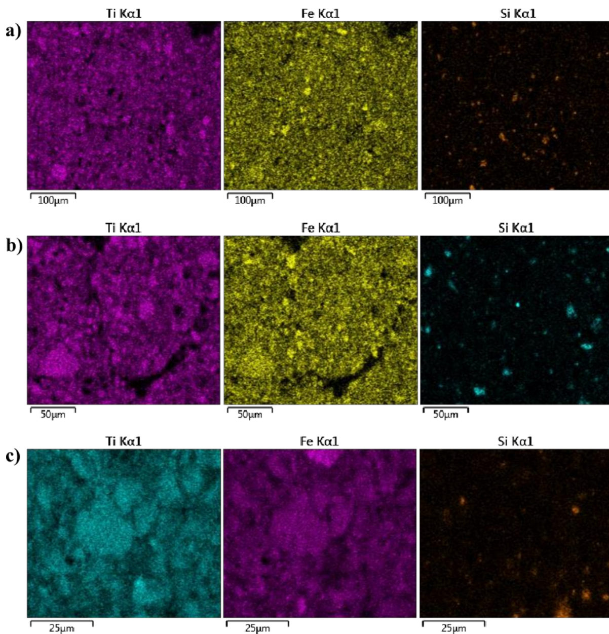
Figure S1. SEM-EDS Micrographs of three different sites (a, b and c) of the catalyst sample using EDS to determine the elemental composition
