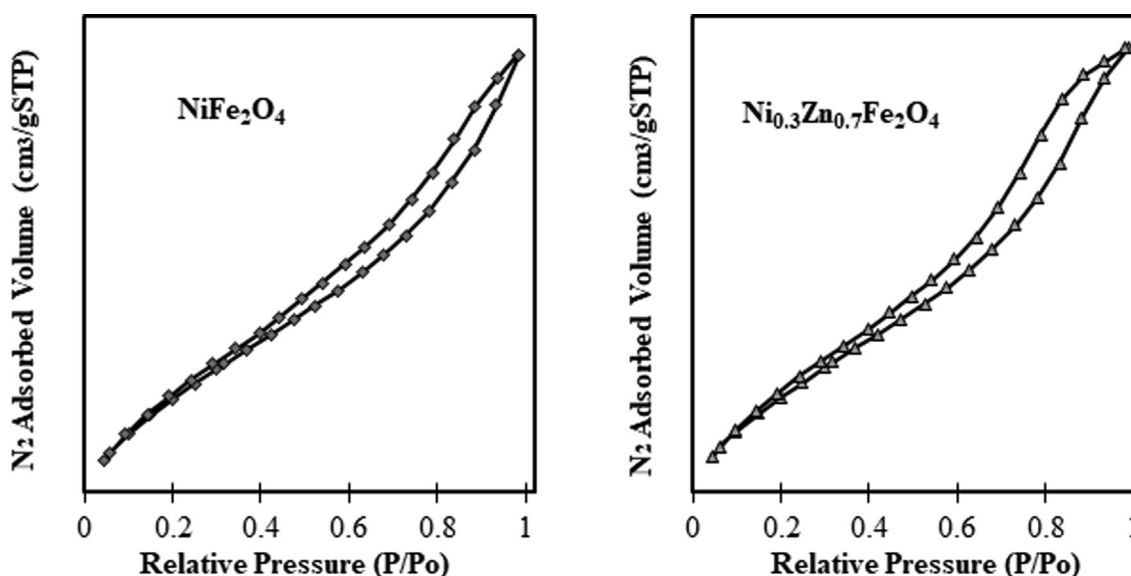
Fig. 4 Adsorption/desorption isotherms of the \text{NiFe}_2\text{O}_4 and \text{Ni}_{0.3}\text{Zn}_{0.7}\text{Fe}_2\text{O}_4 nanocatalysts.
