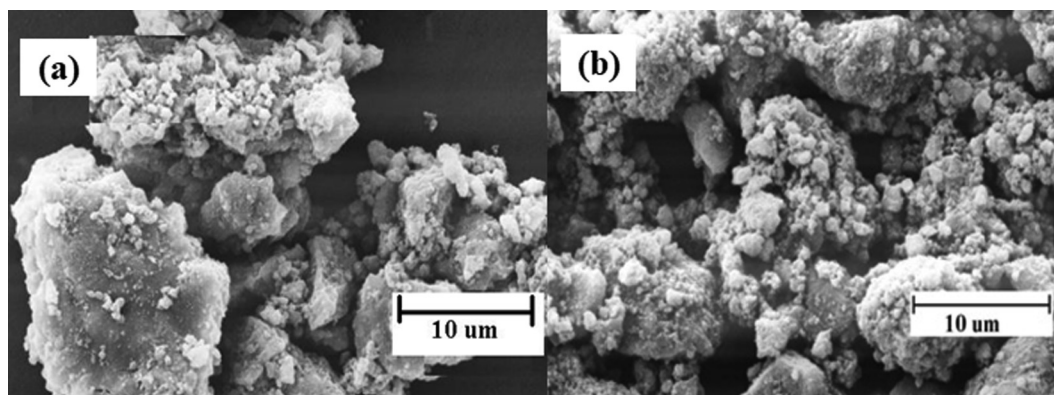
Fig. 6 SEM mesoporous structures of (a) \text{NiFe}_2\text{O}_4 and (b) \text{Ni}_{0.3}\text{Zn}_{0.7}\text{Fe}_2\text{O}_4 ferrites.
