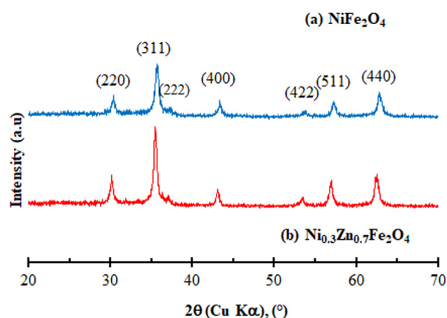
Fig. 1 X-ray diffraction patterns of synthesized (a) NiFe 2 O 4 and (b) Ni 0.3 Zn 0.7 Fe 2 O 4 ferrites.
