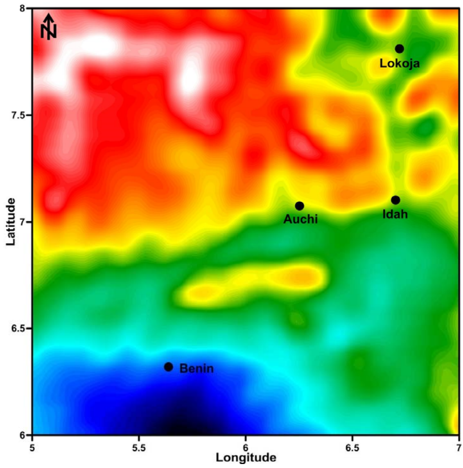
Free-air anomaly map of the study area.
