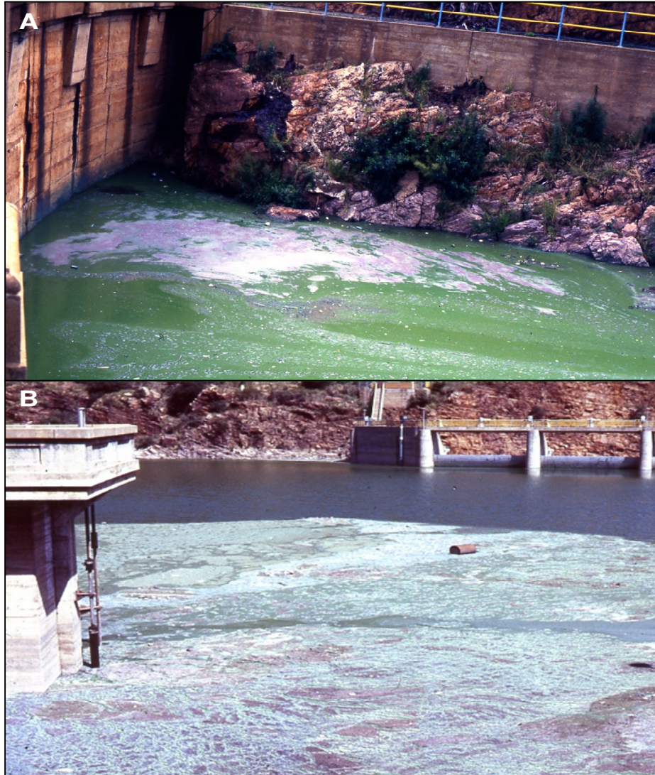
Figure 2. (A) Ground monitoring image showing the formation of white hyperscum crust at the reservoir wall of Lake Hartbeespoort during late February 2005. (B) Ground monitoring image March 26, 2005 showing the distinctive white hyperscum crust at sampling site 1.
