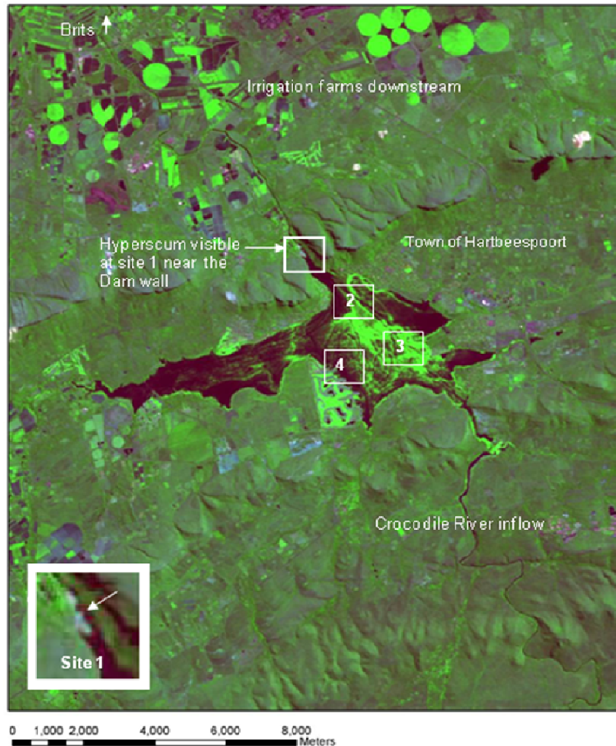
Figure 1. A landsat-5 satellite image of Lake Hartbeespoort taken on March 8, 2005, showing the location of the four sampling sites and the cyanobacterial bloom. Inset shows the distinctive white hyperscum crust at sampling site 1.
